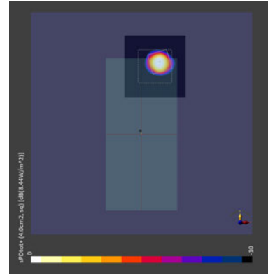
Figure 2-33 Simulated (left) and measured (right) averaged PD distribution for the following configuration: Band n261, MID Channel, Beam ID 3, H polarization, Plane B Module, plotted on the surface S2 (back) with 2mm separation distance to the camera bump.
