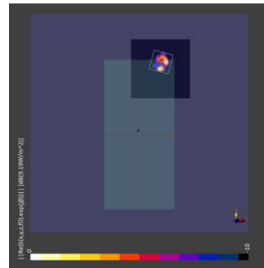
Figure 2-13 Simulated (left) and measured (right) averaged PD distribution for the following configuration: Band n258, MID Channel, Beam ID 2, H+V polarization, Plane B Module, plotted on the surface S2 (back) with 2mm separation distance to the camera bump.
