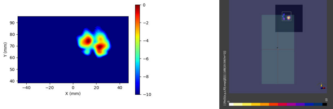
Figure 2-22 Simulated (left) and measured (right) PD distribution for the following configuration: Band n260, MID Channel, Beam ID 3, V polarization, Plane B Module, plotted on the surface S2 (back) with 2mm separation distance to the camera bump.
