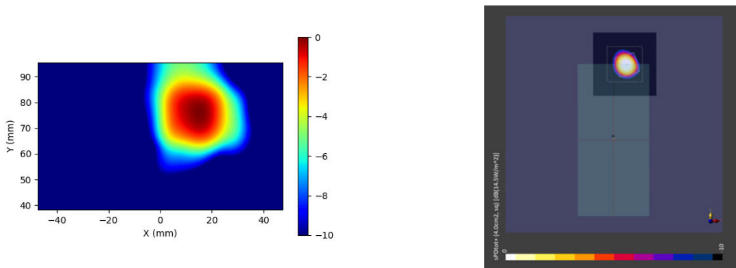
Figure 2-11 Simulated (left) and measured (right) averaged PD distribution for the following configuration: Band n258, MID Channel, Beam ID 2, V polarization, Plane B Module, plotted on the surface S2 (back) with 2mm separation distance to the camera bump.
