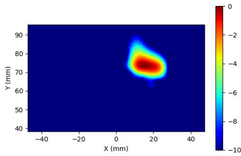
Figure 2-12 Simulated (left) and measured (right) PD distribution for the following configuration: Band n258, MID Channel, Beam ID 2, H+V polarization, Plane B Module, plotted on the surface S2 (back) with 2mm separation distance to the camera bump.
