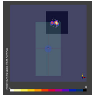
Figure 2-8 Simulated (left) and measured (right) PD distribution for the following configuration: Band n258, MID Channel, Beam ID 4, H polarization, Plane B Module, plotted on the surface S2 (back) with 2mm separation distance to the camera bump.
