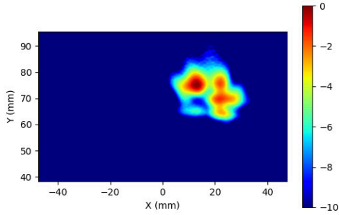
Figure 2-24 Simulated (left) and measured (right) PD distribution for the following configuration: Band n260, MID Channel, Beam ID 3, H+V polarization, Plane B Module, plotted on the surface S2 (back) with 2mm separation distance to the camera bump.
