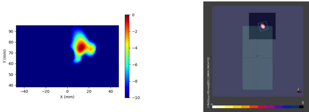
Figure 2-10 Simulated (left) and measured (right) PD distribution for the following configuration: Band n258, MID Channel, Beam ID 2, V polarization, Plane B Module, plotted on the surface S2 (back) with 2mm separation distance to the camera bump.
