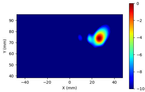
Figure 2-36 Simulated (left) and measured (right) PD distribution for the following configuration: Band n261, MID Channel, Beam ID 5, H+V polarization, Plane B Module, plotted on the surface S2 (back) with 2mm separation distance to the camera bump.
