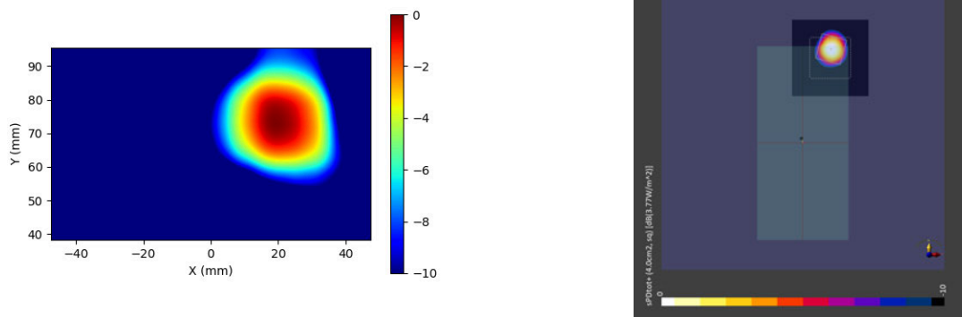
Figure 2-21 Simulated (left) and measured (right) averaged PD distribution for the following configuration: Band n260, MID Channel, Beam ID 4, H polarization, Plane B Module, plotted on the surface S2 (back) with 2mm separation distance to the camera bump.
