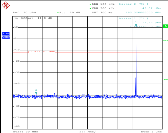
Conducted Spurious Emission Plot on Bluetooth LE 2Mbps GFSK Channel 39
