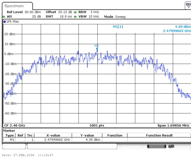
Power Density (dBm/3kHz) Plot Channel 78
