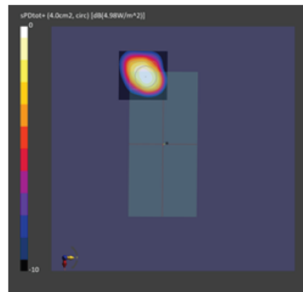
Figure 2-33 Simulated (left) and measured (right) averaged PD distribution for the following configuration: Band n261, MID Channel, Beam ID 1, H polarization, Plane-B Module, plotted on the surface S2 (back) with 10mm separation distance to the camera bump.
