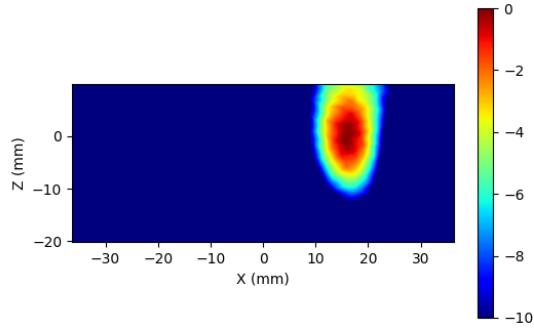
Figure 2-24 Simulated (left) and measured (right) PD distribution for the following configuration: Band n261, MID Channel, Beam ID 3, H+V polarization, Plane-A Module, plotted on the surface S5 (top) with 10mm separation distance to the DUT.
