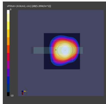
Figure 2-3 Simulated (left) and measured (right) averaged PD distribution for the following configuration: Band n260, MID Channel, Beam ID 0, H polarization, Plane-A Module, plotted on the surface S5 (top) with 10mm separation distance to the DUT.
