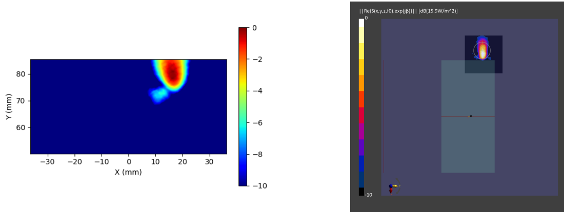
Figure 2-28 Simulated (left) and measured (right) PD distribution for the following configuration: Band n261, MID Channel, Beam ID 3, V polarization, Plane-A Module, plotted on the surface S1 (Front) with 2mm separation distance to the DUT.
