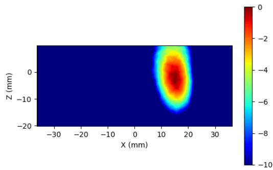
Figure 2-20 Simulated (left) and measured (right) PD distribution for the following configuration: Band n261, MID Channel, Beam ID 2, H polarization, Plane-A Module, plotted on the surface S5 (top) with 10mm separation distance to the DUT.
