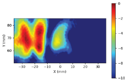
Figure 2-32 Simulated (left) and measured (right) PD distribution for the following configuration: Band n261, MID Channel, Beam ID 1, H polarization, Plane-B Module, plotted on the surface S2 (back) with 10mm separation distance to the camera bump.
