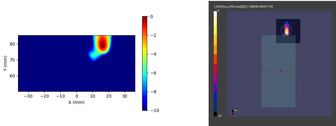
Figure 2-30 Simulated (left) and measured (right) PD distribution for the following configuration: Band n261, MID Channel, Beam ID 3, H+V polarization, Plane-A Module, plotted on the surface S1 (Front) with 2mm separation distance to the DUT.
