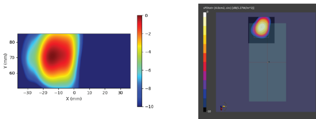
Figure 2-35 Simulated (left) and measured (right) averaged PD distribution for the following configuration: Band n261, MID Channel, Beam ID 4, V polarization, Plane-B Module, plotted on the surface S2 (back) with 10mm separation distance to the camera bump.
