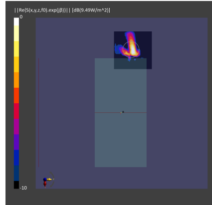
Figure 2-8 Simulated (left) and measured (right) PD distribution for the following configuration: Band n260, MID Channel, Beam ID 2, H polarization, Plane-A Module, plotted on the surface S1 (Front) with 2mm separation distance to the DUT.
