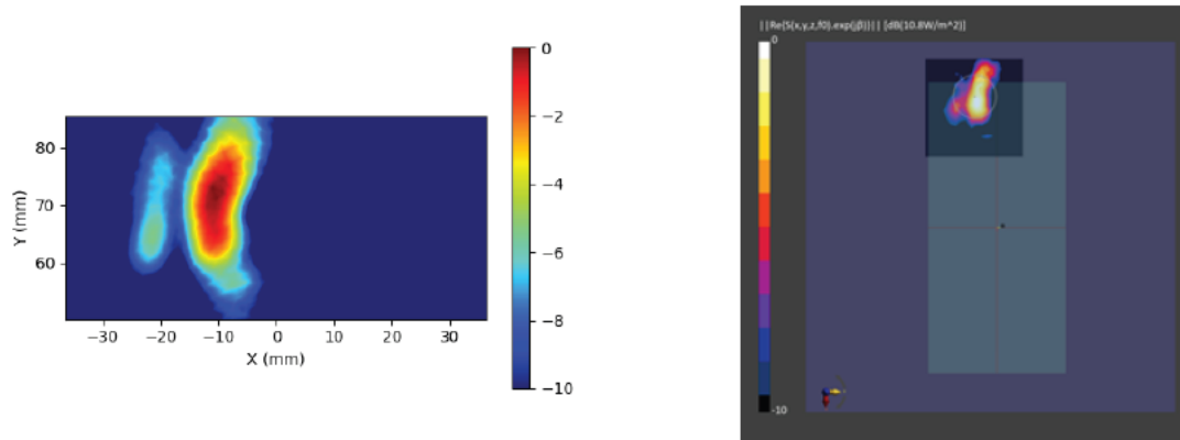
Figure 2-34 Simulated (left) and measured (right) PD distribution for the following configuration: Band n261, MID Channel, Beam ID 4, V polarization, Plane-B Module, plotted on the surface S2 (back) with 10mm separation distance to the camera bump.
