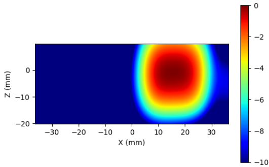
Figure 2-23 Simulated (left) and measured (right) averaged PD distribution for the following configuration: Band n261, MID Channel, Beam ID 3, V polarization, Plane-A Module, plotted on the surface S5 (top) with 10mm separation distance to the DUT.
