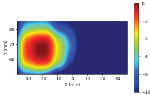
Figure 2-19 Simulated (left) and measured (right) averaged PD distribution for the following configuration: Band n260, MID Channel, Beam ID 1, H+V polarization, Plane-B Module, plotted on the surface S2 (back) with 10mm separation distance to the camera bump.
