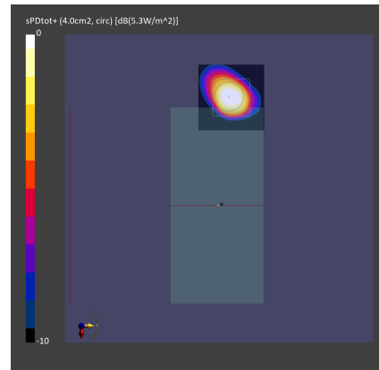
Figure 2-27 Simulated (left) and measured (right) averaged PD distribution for the following configuration: Band n261, MID Channel, Beam ID 0, H polarization, Plane-A Module, plotted on the surface S1 (Front) with 2mm separation distance to the DUT.
