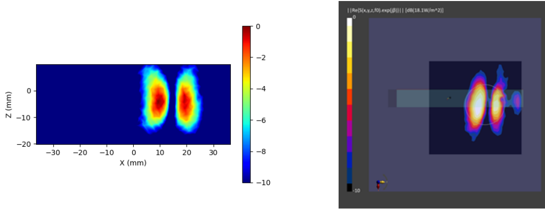
Figure 2-6 Simulated (left) and measured (right) PD distribution for the following configuration: Band n260, MID Channel, Beam ID 1, H+V polarization, Plane-A Module, plotted on the surface S5 (top) with 10mm separation distance to the DUT.
