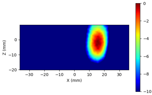
Figure 2-22 Simulated (left) and measured (right) PD distribution for the following configuration: Band n261, MID Channel, Beam ID 3, V polarization, Plane-A Module, plotted on the surface S5 (top) with 10mm separation distance to the DUT.
