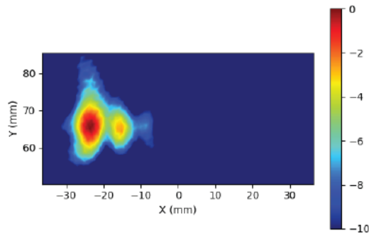
Figure 2-18 Simulated (left) and measured (right) PD distribution for the following configuration: Band n260, MID Channel, Beam ID 1, H+V polarization, Plane-B Module, plotted on the surface S2 (back) with 10mm separation distance to the camera bump.
