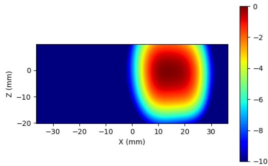
Figure 2-21 Simulated (left) and measured (right) averaged PD distribution for the following configuration: Band n261, MID Channel, Beam ID 2, H polarization, Plane-A Module, plotted on the surface S5 (top) with 10mm separation distance to the DUT.
