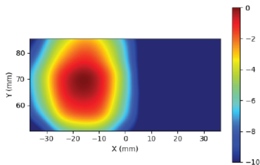
Figure 2-37 Simulated (left) and measured (right) averaged PD distribution for the following configuration: Band n261, MID Channel, Beam ID 3, H+V polarization, Plane-B Module, plotted on the surface S2 (back) with 10mm separation distance to the camera bump.
