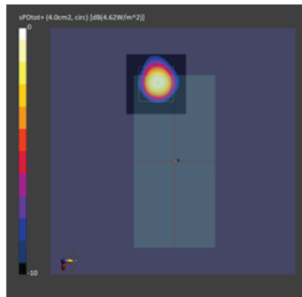
Figure 2-17 Simulated (left) and measured (right) averaged PD distribution for the following configuration: Band n260, MID Channel, Beam ID 3, V polarization, Plane-B Module, plotted on the surface S2 (back) with 10mm separation distance to the camera bump.
