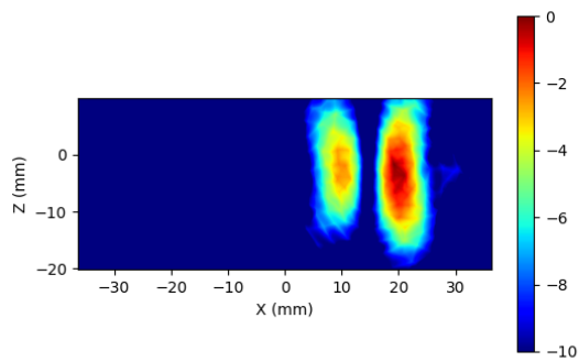
Figure 2-4 Simulated (left) and measured (right) PD distribution for the following configuration: Band n260, MID Channel, Beam ID 1, V polarization, Plane-A Module, plotted on the surface S5 (top) with 10mm separation distance to the DUT.
