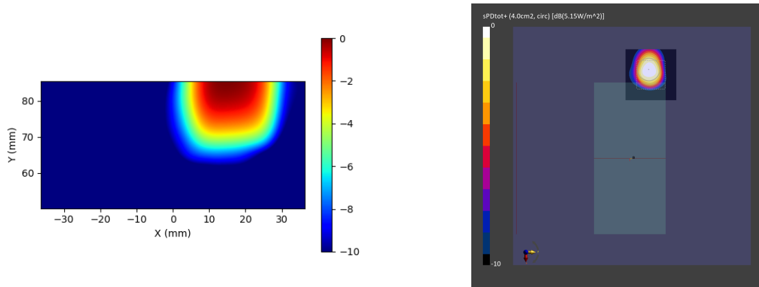
Figure 2-29 Simulated (left) and measured (right) averaged PD distribution for the following configuration: Band n261, MID Channel, Beam ID 3, V polarization, Plane-A Module, plotted on the surface S1 (Front) with 2mm separation distance to the DUT.
