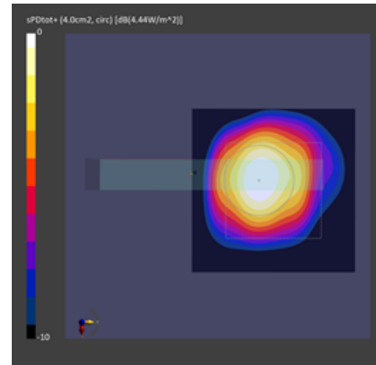
Figure 2-5 Simulated (left) and measured (right) averaged PD distribution for the following configuration: Band n260, MID Channel, Beam ID 1, V polarization, Plane-A Module, plotted on the surface S5 (top) with 10mm separation distance to the DUT.
