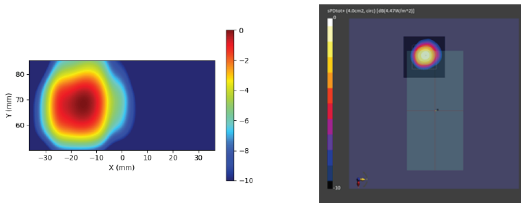
Figure 2-15 Simulated (left) and measured (right) averaged PD distribution for the following configuration: Band n260, MID Channel, Beam ID 3, H polarization, Plane-B Module, plotted on the surface S2 (back) with 10mm separation distance to the camera bump.
