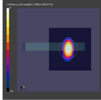
Figure 2-22 Simulated (left) and measured (right) PD distribution for the following configuration: Band n261, MID Channel, Beam ID 3, V polarization, Plane-A Module, plotted on the surface S5 (top) with 10mm separation distance to the DUT.
