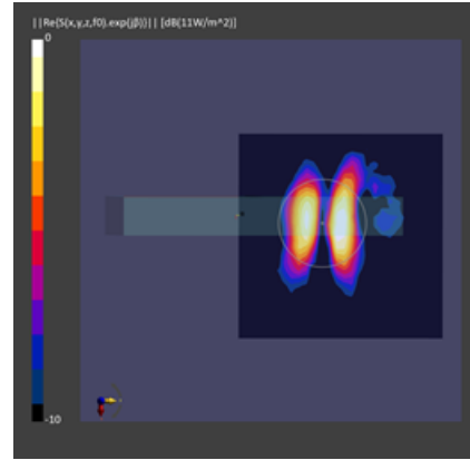
Figure 2-4 Simulated (left) and measured (right) PD distribution for the following configuration: Band n260, MID Channel, Beam ID 1, V polarization, Plane-A Module, plotted on the surface S5 (top) with 10mm separation distance to the DUT.
