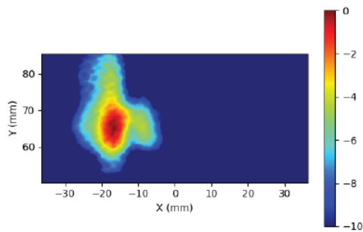
Figure 2-16 Simulated (left) and measured (right) PD distribution for the following configuration: Band n260, MID Channel, Beam ID 3, V polarization, Plane-B Module, plotted on the surface S2 (back) with 10mm separation distance to the camera bump.
