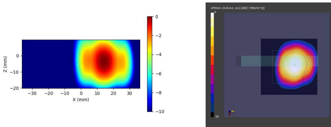
Figure 2-7 Simulated (left) and measured (right) averaged PD distribution for the following configuration: Band n260, MID Channel, Beam ID 1, H+V polarization, Plane-A Module, plotted on the surface S5 (top) with 10mm separation distance to the DUT.
