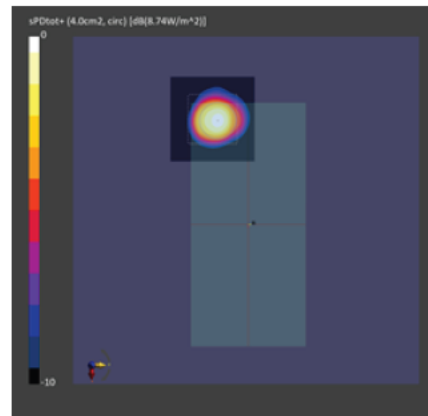
Figure 2-19 Simulated (left) and measured (right) averaged PD distribution for the following configuration: Band n260, MID Channel, Beam ID 1, H+V polarization, Plane-B Module, plotted on the surface S2 (back) with 10mm separation distance to the camera bump.
