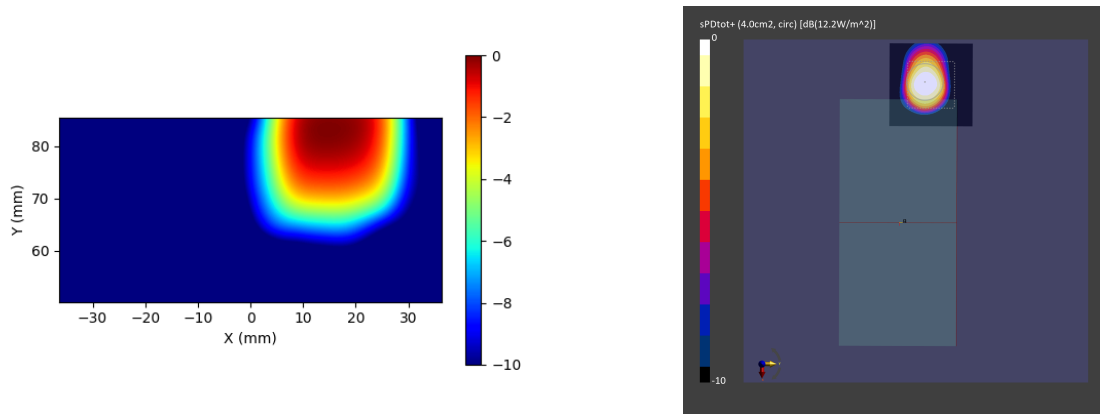
Figure 2-31 Simulated (left) and measured (right) averaged PD distribution for the following configuration: Band n261, MID Channel, Beam ID 3, H+V polarization, Plane-A Module, plotted on the surface S1 (Front) with 2mm separation distance to the DUT.
