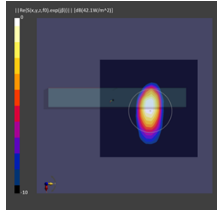
Figure 2-24 Simulated (left) and measured (right) PD distribution for the following configuration: Band n261, MID Channel, Beam ID 3, H+V polarization, Plane-A Module, plotted on the surface S5 (top) with 10mm separation distance to the DUT.
