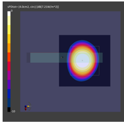
Figure 2-23 Simulated (left) and measured (right) averaged PD distribution for the following configuration: Band n261, MID Channel, Beam ID 3, V polarization, Plane-A Module, plotted on the surface S5 (top) with 10mm separation distance to the DUT.
