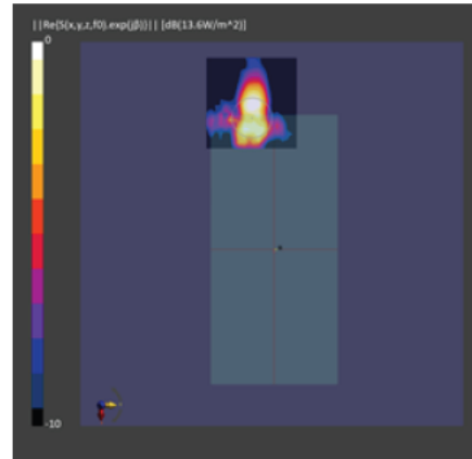
Figure 2-36 Simulated (left) and measured (right) PD distribution for the following configuration: Band n261, MID Channel, Beam ID 3, H+V polarization, Plane-B Module, plotted on the surface S2 (back) with 10mm separation distance to the camera bump.
