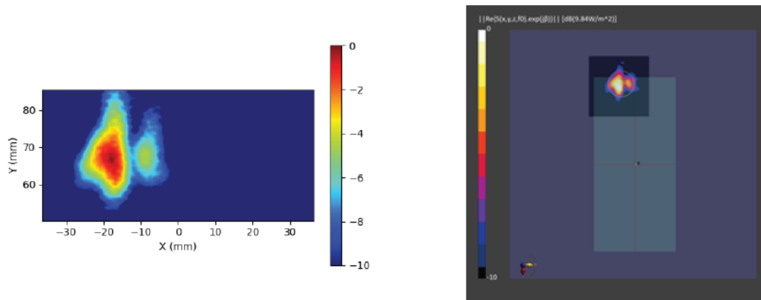
Figure 2-14 Simulated (left) and measured (right) PD distribution for the following configuration: Band n260, MID Channel, Beam ID 3, H polarization, Plane-B Module, plotted on the surface S2 (back) with 10mm separation distance to the camera bump.
