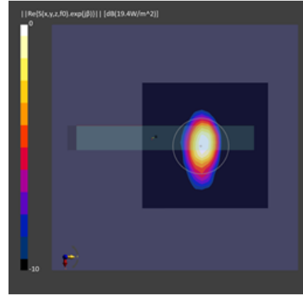
Figure 2-20 Simulated (left) and measured (right) PD distribution for the following configuration: Band n261, MID Channel, Beam ID 2, H polarization, Plane-A Module, plotted on the surface S5 (top) with 10mm separation distance to the DUT.
