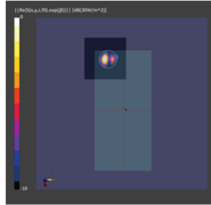
Figure 2-18 Simulated (left) and measured (right) PD distribution for the following configuration: Band n260, MID Channel, Beam ID 1, H+V polarization, Plane-B Module, plotted on the surface S2 (back) with 10mm separation distance to the camera bump.
