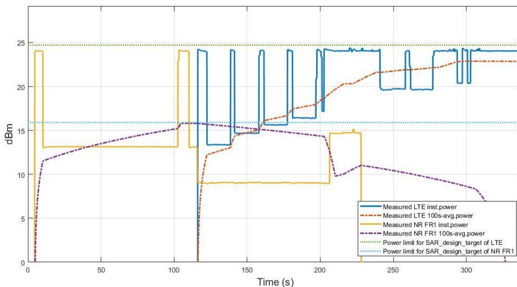
Figure 6.8-1 Time average SAR of LTE B25/2 and FR1 n38 in EN-DC case
