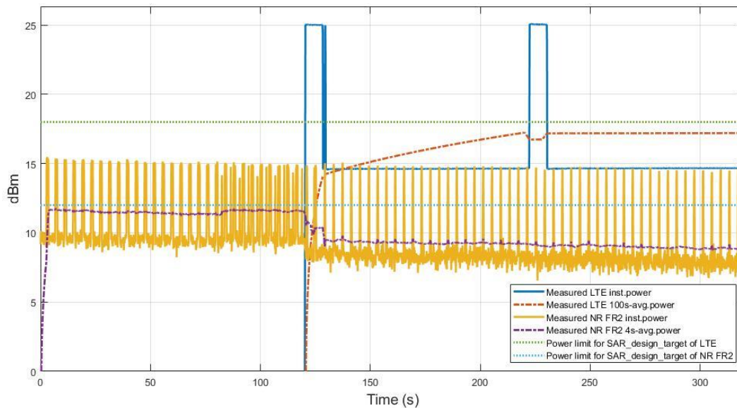
Figure 7.2-1 Conducted power of LTE B7 and radiated EIRP of FR2 n258 in EN-DC max power
