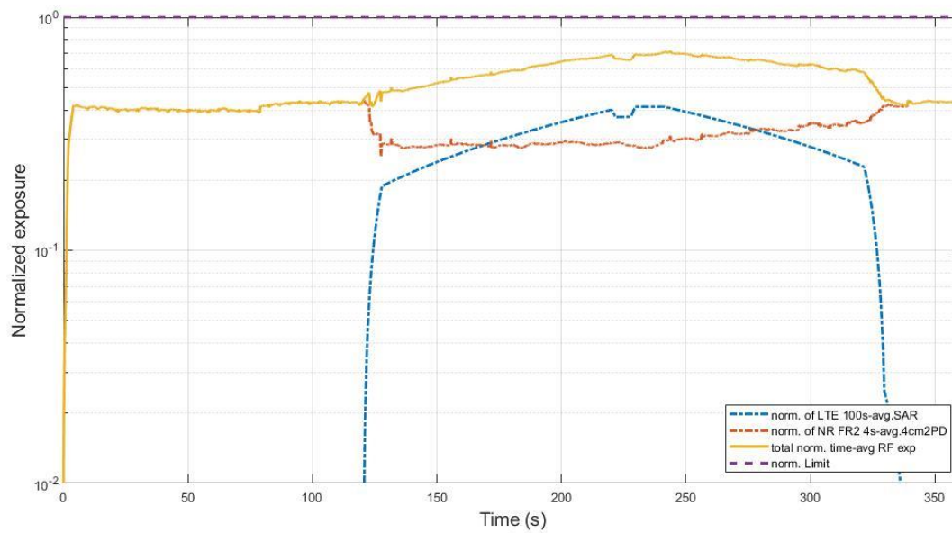
Figure 7.3-2 Total normalized time-average RF exposure in F_TC02
