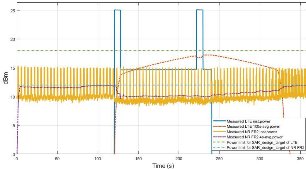
Figure 7.3-1 Conducted power of LTE B7 and radiated EIRP of FR2 n258 in EN-DC max power case
