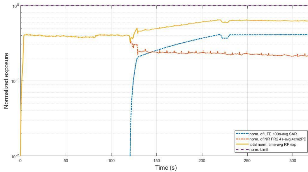
Figure 7.2-2 Total normalized time-average RF exposure in F_TC01
