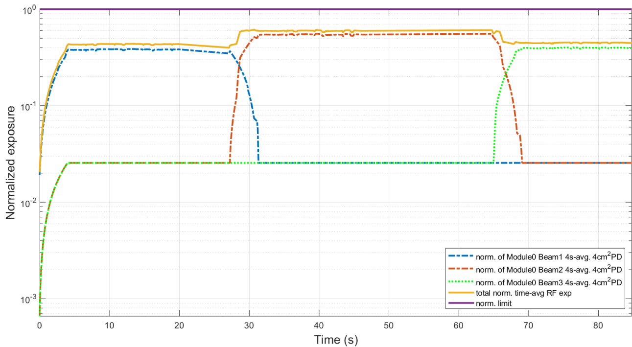
Figure 7.4-2 Total normalized time-average RF exposure
