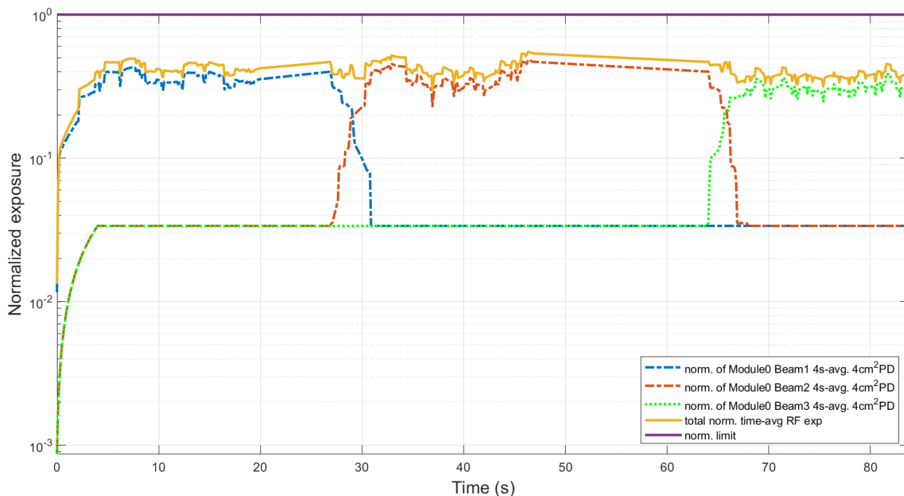
Figure 7.7-2 Total normalized time-average RF exposure
