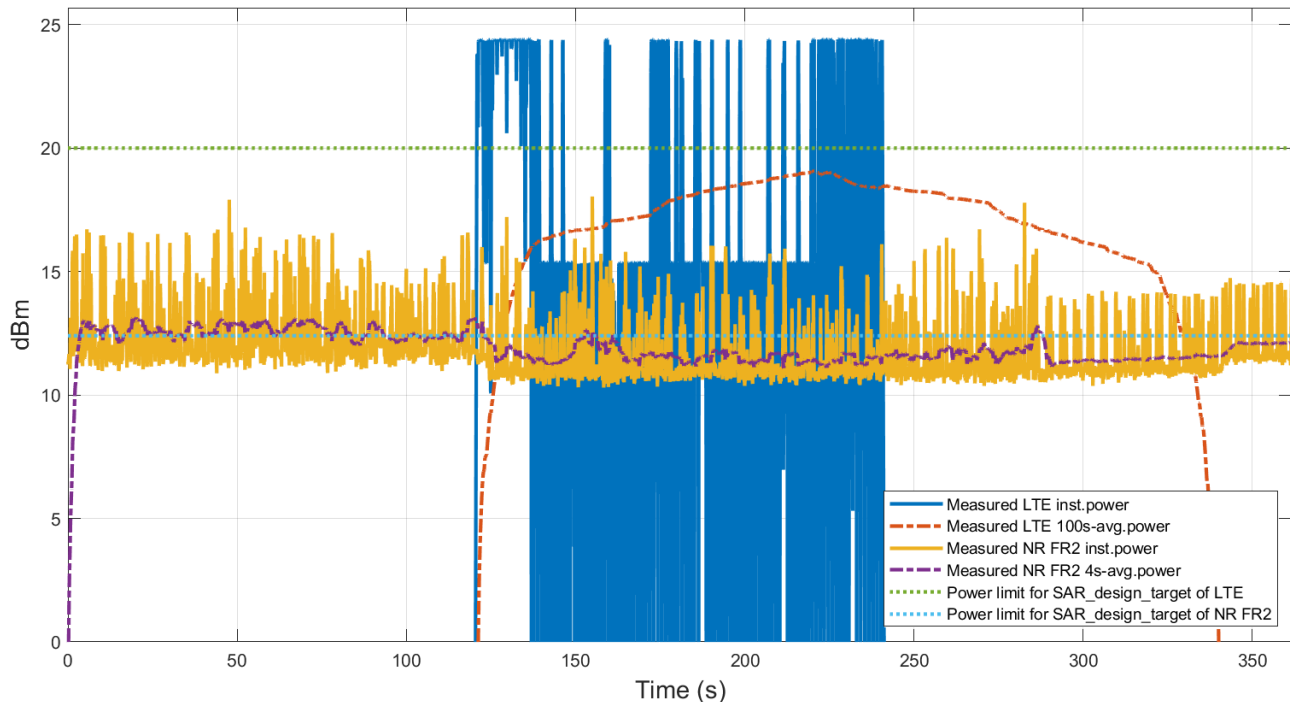
Figure 7.3-1 Conducted power of LTE B2 and radiated EIRP of FR2 n260 in EN-DC max power case
