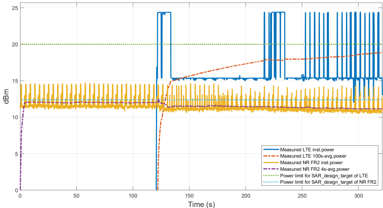
Figure 7.2-1 Conducted power of LTE B2 and radiated EIRP of FR2 n260 in EN-DC max power
