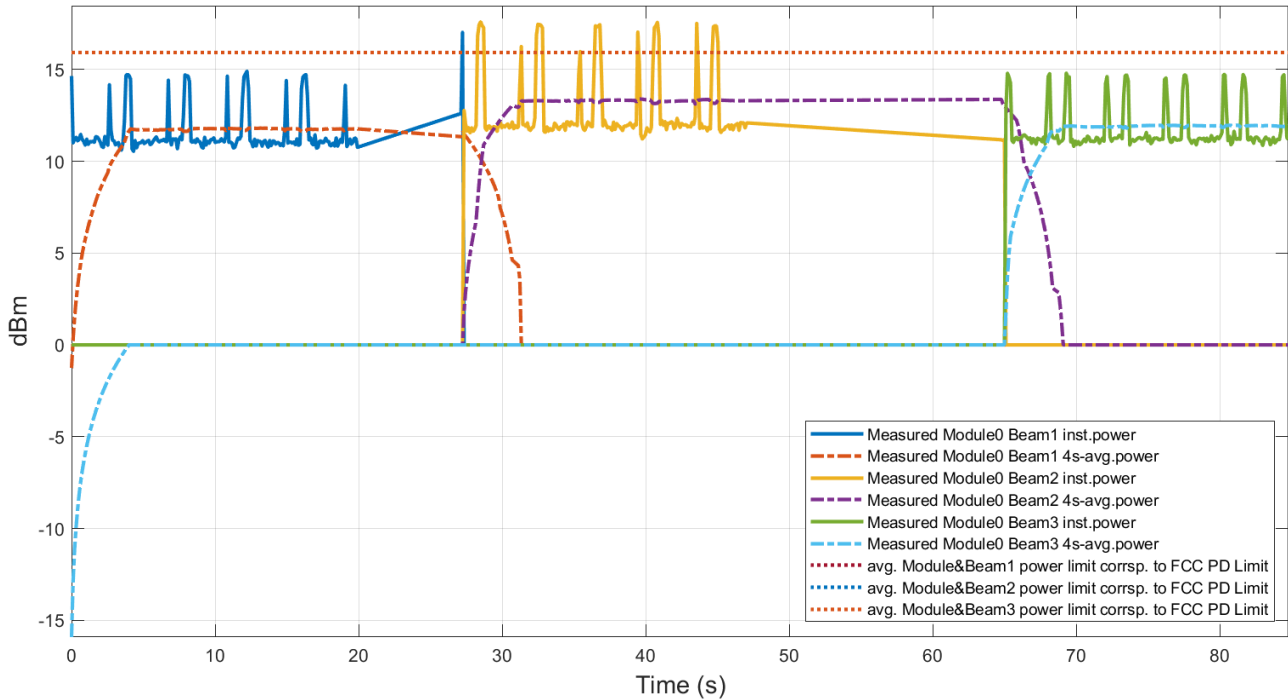
Figure 7.4-1 Measured radiated EIRP of FR2 n260 in mmWave Module beam change case F_TC03
