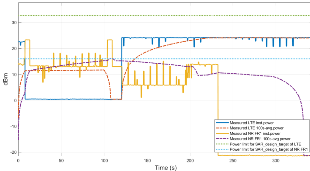
Figure 6.7-1 Time average SAR of LTE B25 and FR1 n41 in EN-DC case
