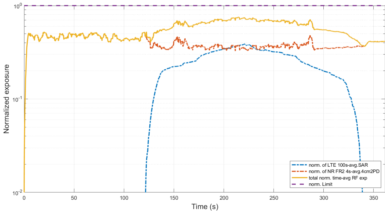
Figure 7.3-2 Total normalized time-average RF exposure in F_TC02
