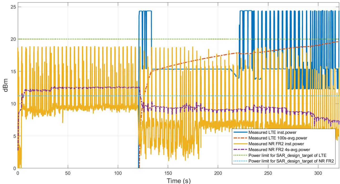
Figure 7.5-1 Conducted power of LTE B2 and radiated EIRP of FR2 n261 in EN-DC max power
