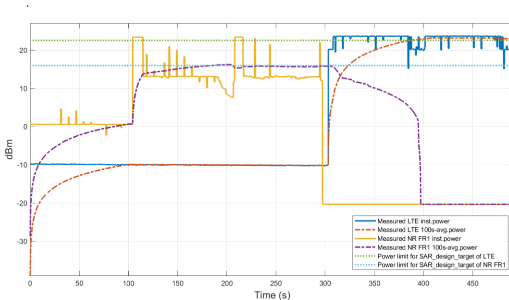
Figure 6.5-1 Conducted Tx power for SAR IRAT re-selection
