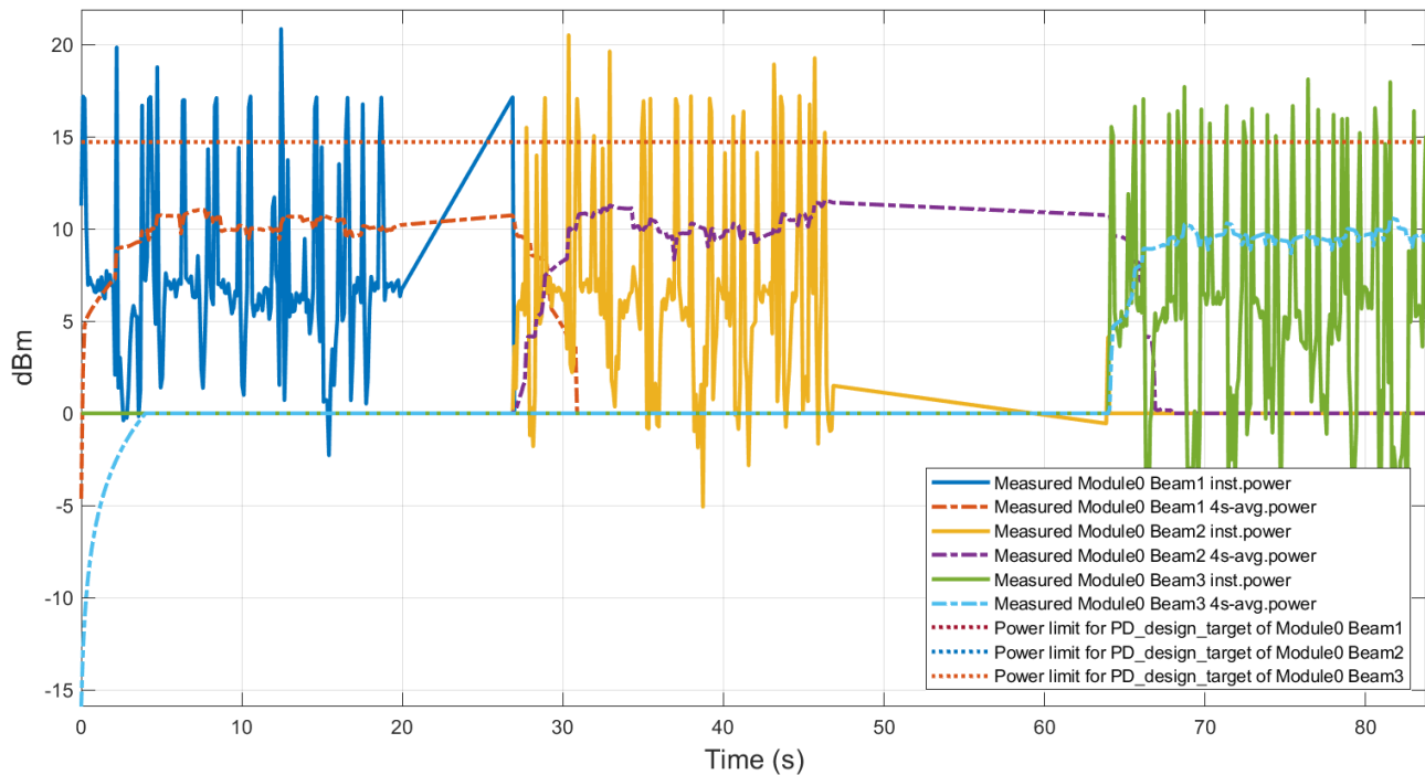
Figure 7.7-1 Measured radiated EIRP of FR2 n260 in mmWave Module beam change case F_TC06
