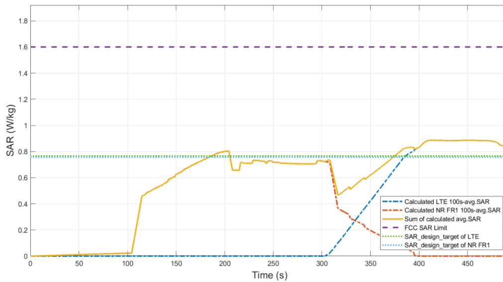
Figure 6.5-2 Total time-averaged SAR
