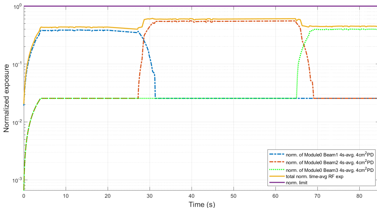
Figure 7.4-2 Total normalized time-average RF exposure
