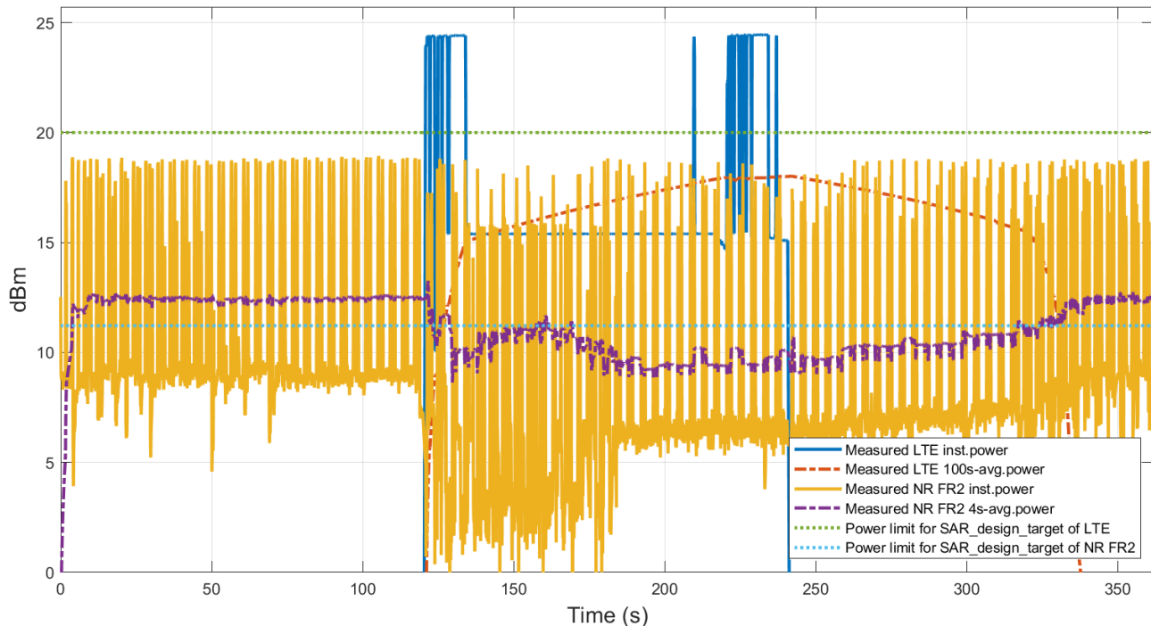
Figure 7.6-1 Conducted power of LTE B2 and radiated EIRP of FR2 n261 in EN-DC max power case
