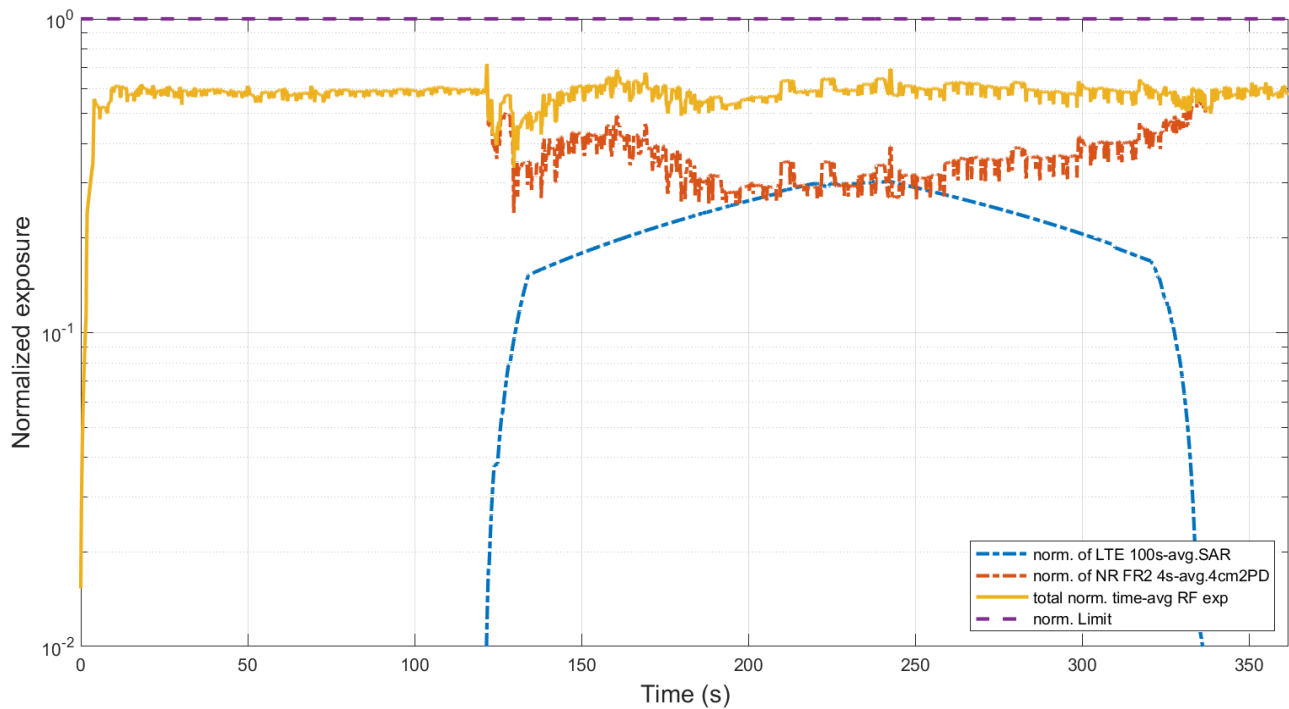
Figure 7.6-2 Total normalized time-average RF exposure in F_TC05
