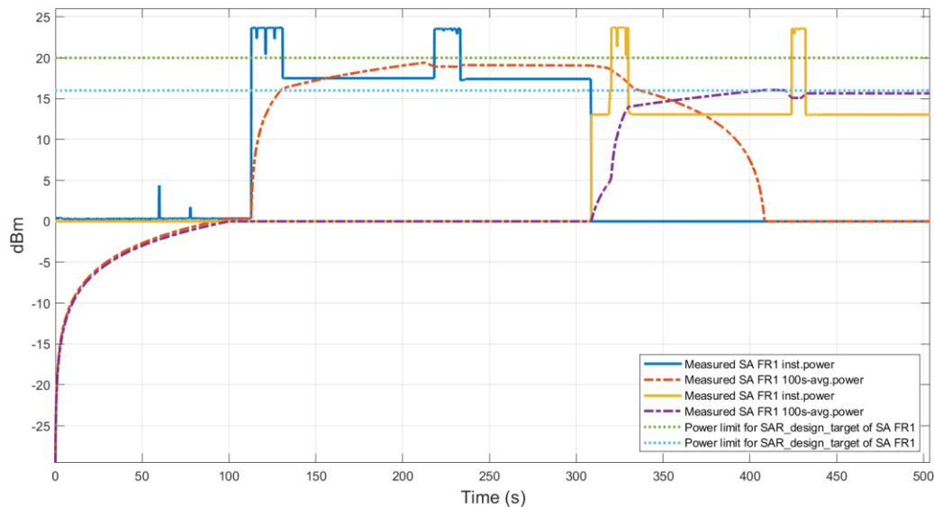
Figure 6.8-1 Conducted Tx power for SAR states change
