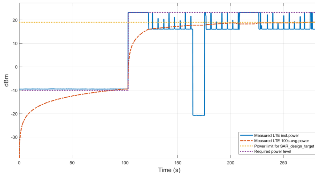
Figure 6.4-1 Conducted Tx power in Call_Disconnect_Reestablishment
