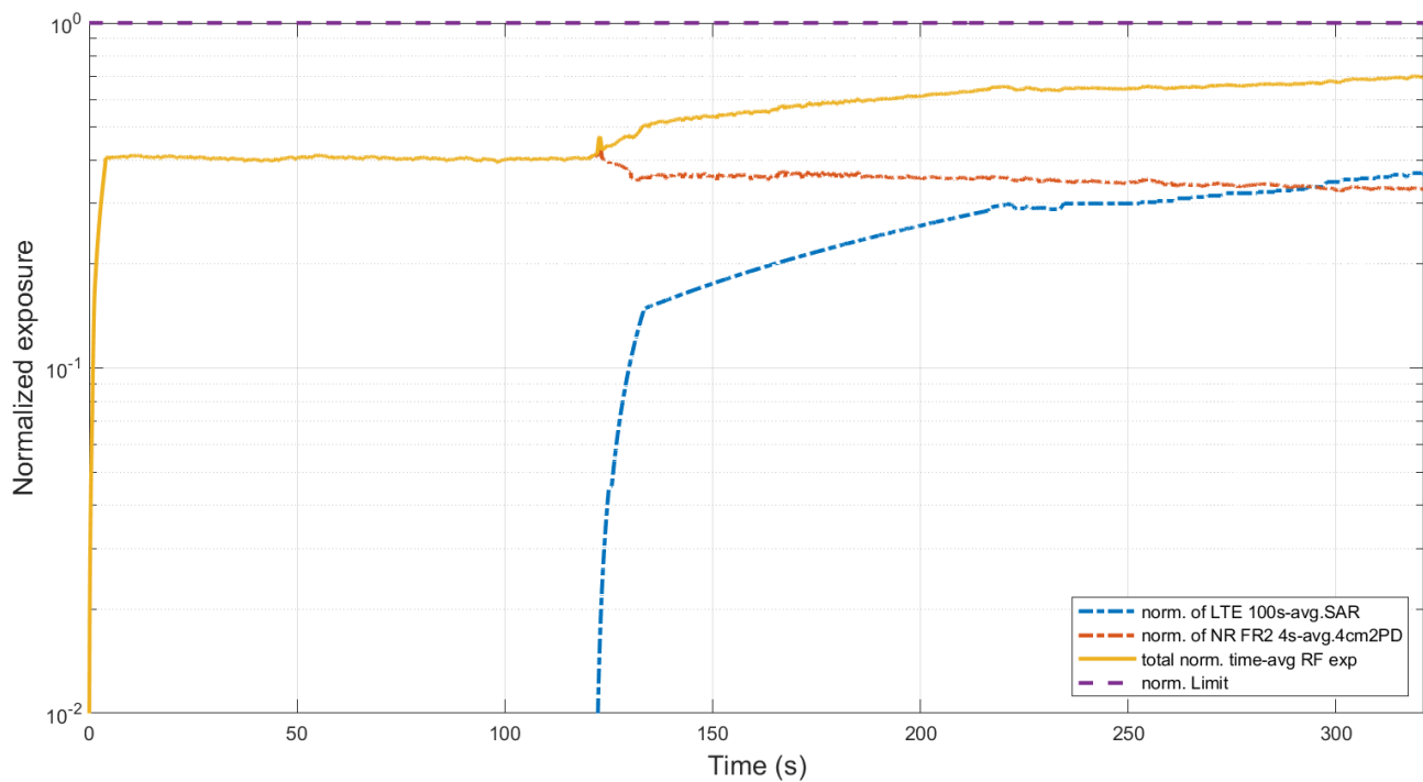
Figure 7.2-2 Total normalized time-average RF exposure in F_TC01
