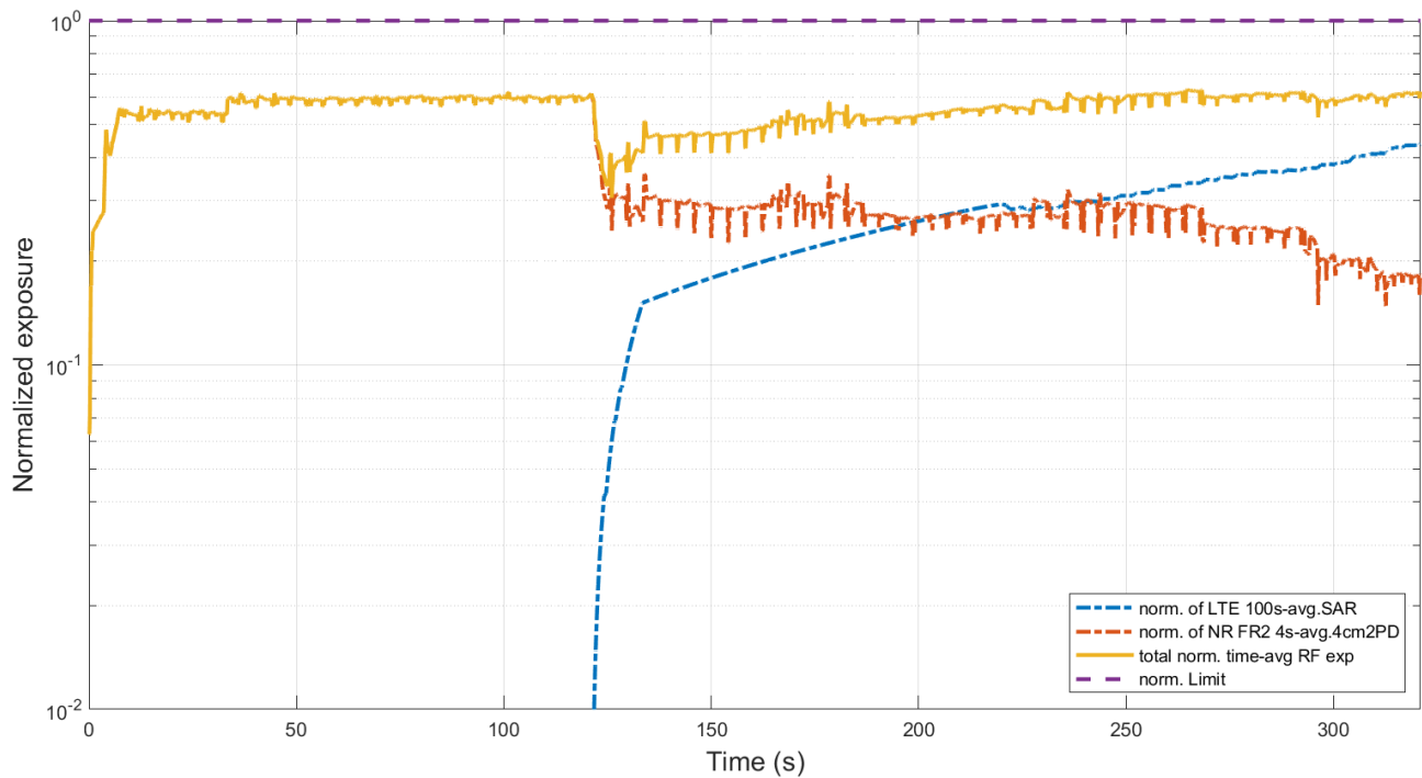
Figure 7.5-2 Total normalized time-average RF exposure in F_TC04
