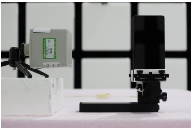
Position D, test separation 15 cm
