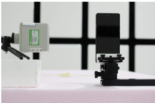
Position C, test separation 15 cm
