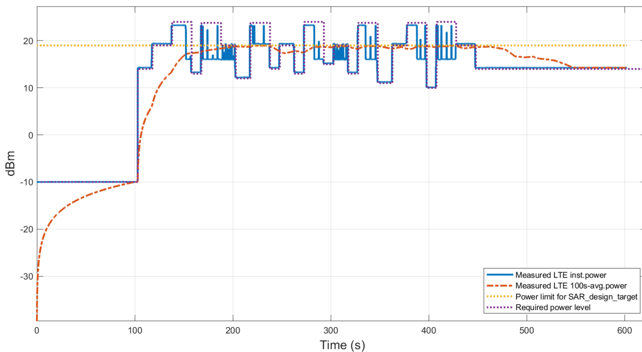
Figure 6.3-5 Conducted Tx power
