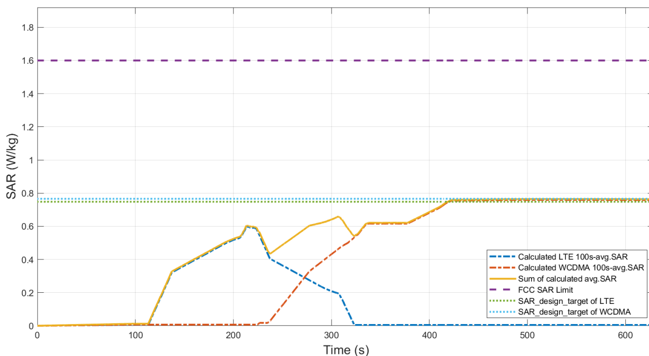
Figure 6.5-2 Total time-averaged SAR
