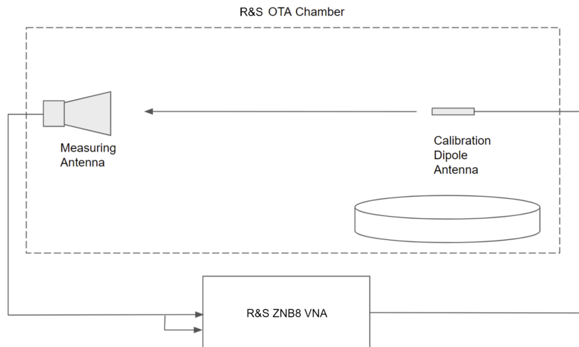
Figure: Chamber Block Diagram of Path Loss
