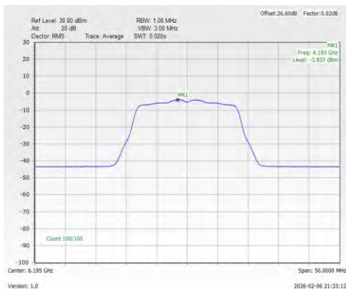
Power Density Plot Trace 1 (Ant 3)
