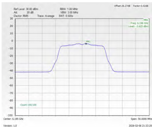
Power Density Plot Trace 2 (Ant 4)
