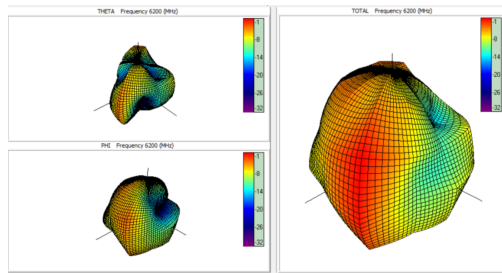
Ant4 Freq. 6175 MHz:
