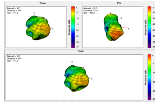
Ant3 Freq. 2462 MHz:
