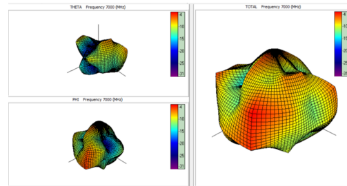
Ant4 Freq. 7000 MHz:
