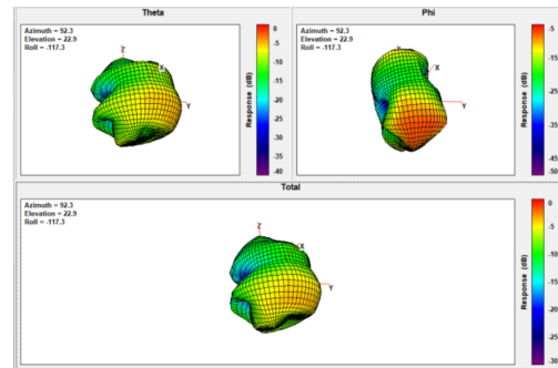
Ant3 Freq. 2437 MHz:
