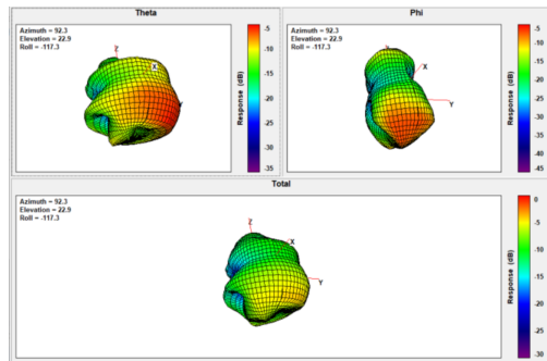
Ant3 Freq. 2402 MHz:
