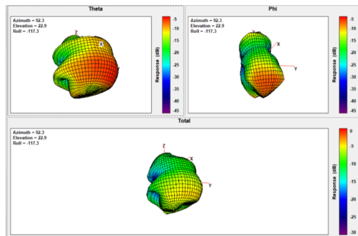
Ant3 Freq. 2412 MHz:
