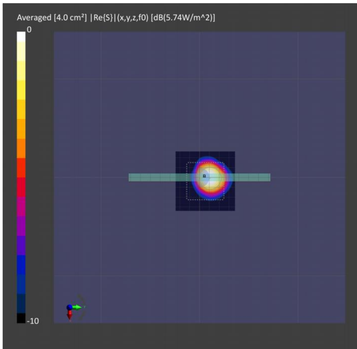
Figure 7-3: 4cm 2 -averaged power density distribution measured at input.power.limit of 4.72 dBm on the Right Side for n260 beam 13
