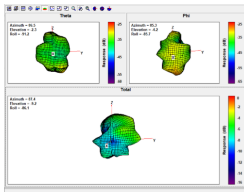
Ant4 Freq. 5500 MHz:
