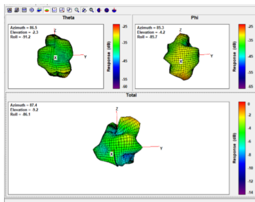
Ant4 Freq. 5820 MHz:
