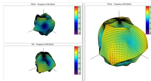
Ant4 Freq. 6700 MHz:
