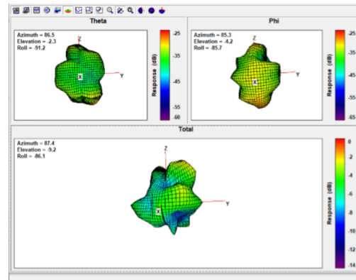
Ant4 Freq. 5887 MHz:
