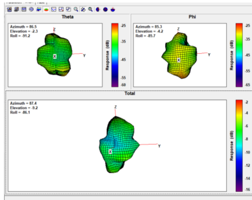
Ant4 Freq. 5280 MHz:
