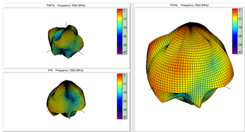
Ant4 Freq. 7000 MHz:
