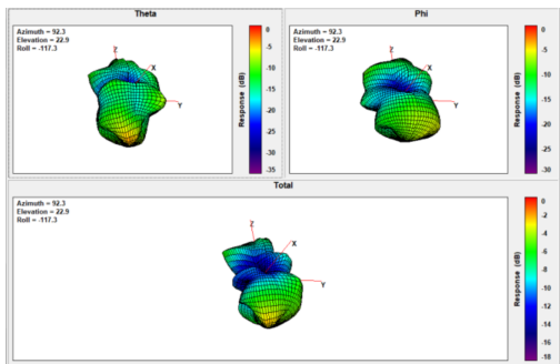
Ant3 Freq. 5180 MHz:
