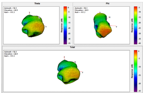
Ant3 Freq. 2462 MHz:
