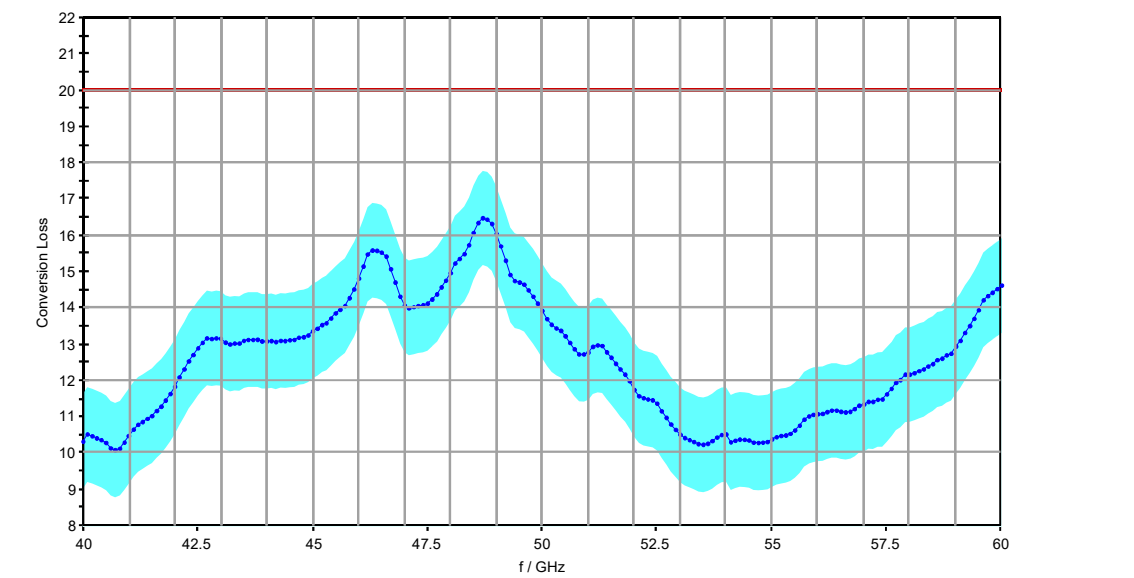
Conversion Loss (IF = 1330 MHz)
