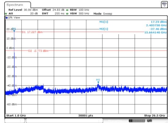
CSE Plot on Low Ch between 1GHz ~ 26.5GHz
