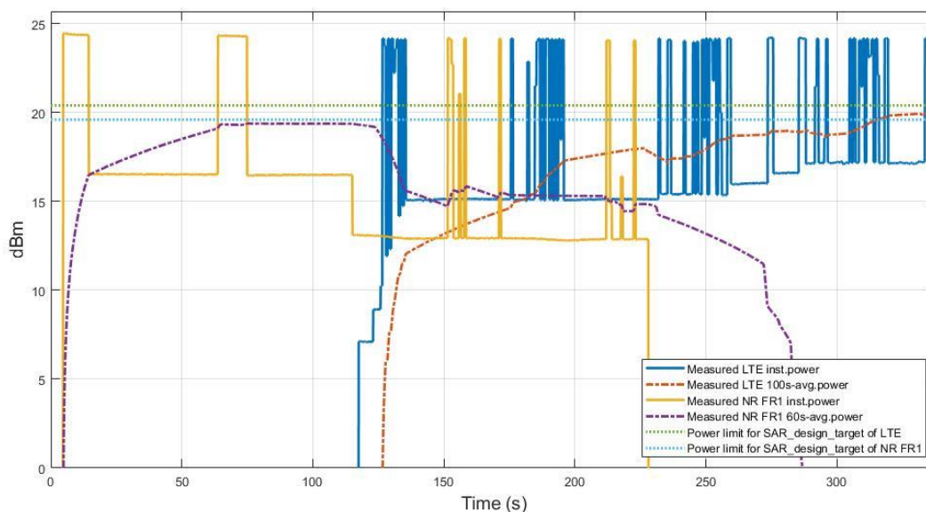
Figure 6.8-1 Time average SAR of LTE B7 and FR1 n77 in EN-DC case
