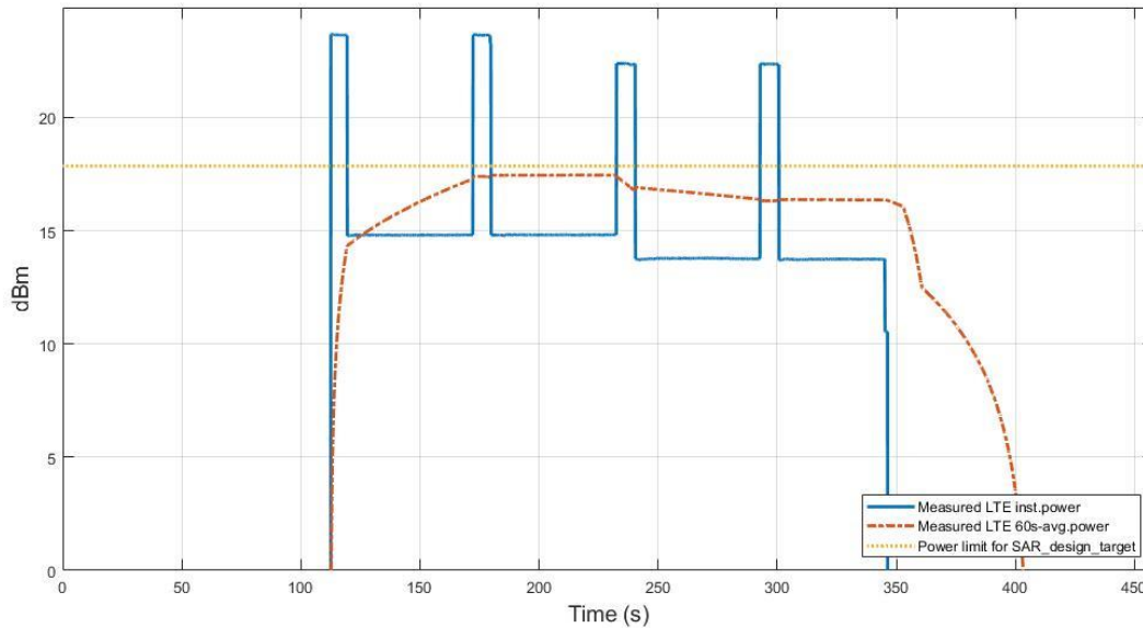
Figure 7.9-1 Conducted transmitted power of LTE B66 in UL CA
