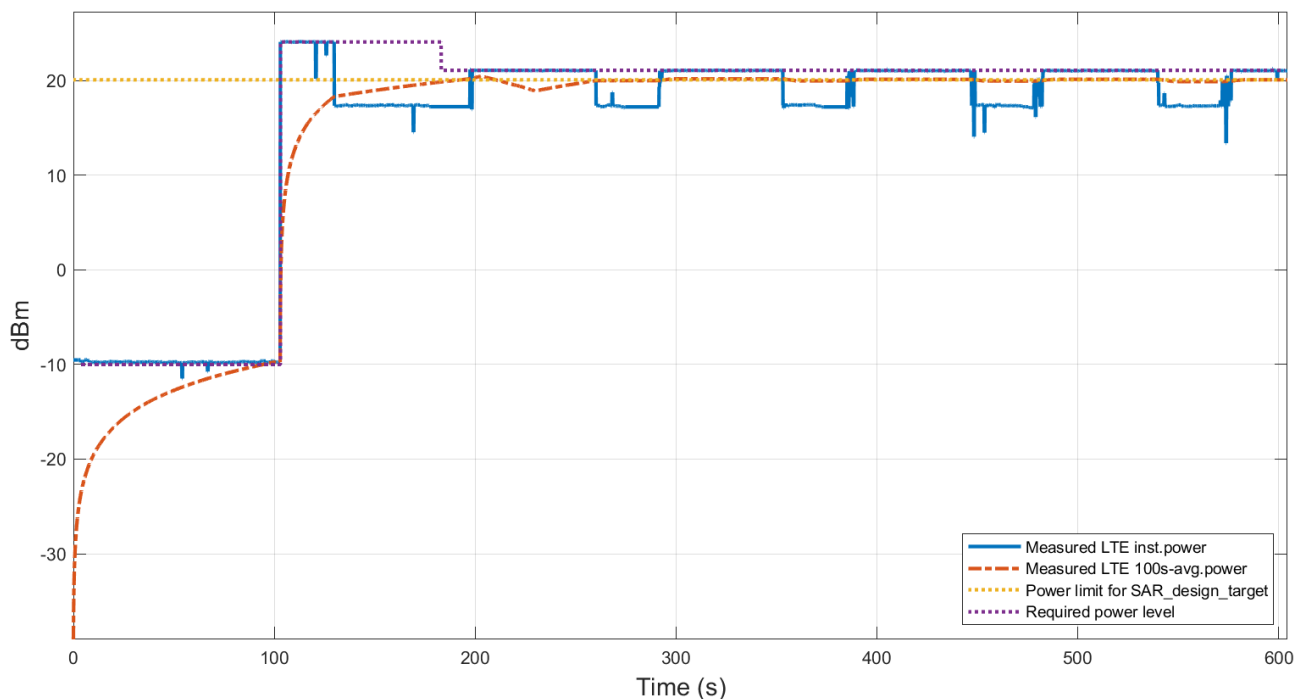
Figure 6.3-1 Time average conducted power
