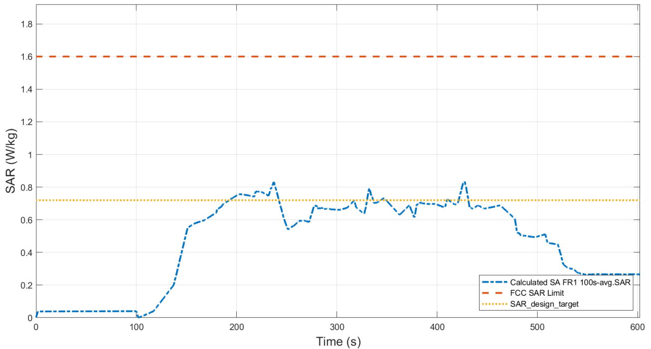
Figure 6.3-8 Total time-averaged SAR in F_TC04
