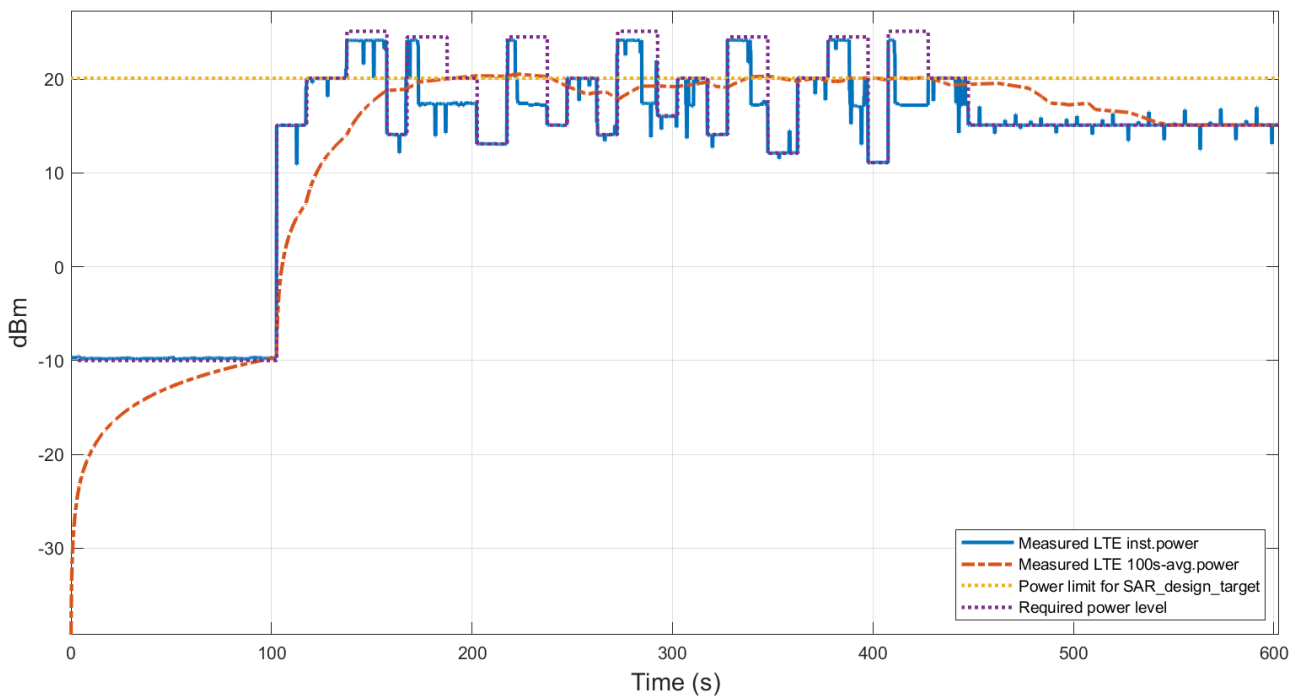
Figure 6.3-5 Conducted Tx power
