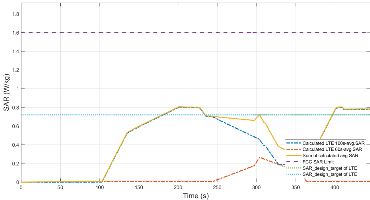
Figure 6.6-2 Total time-averaged SAR
