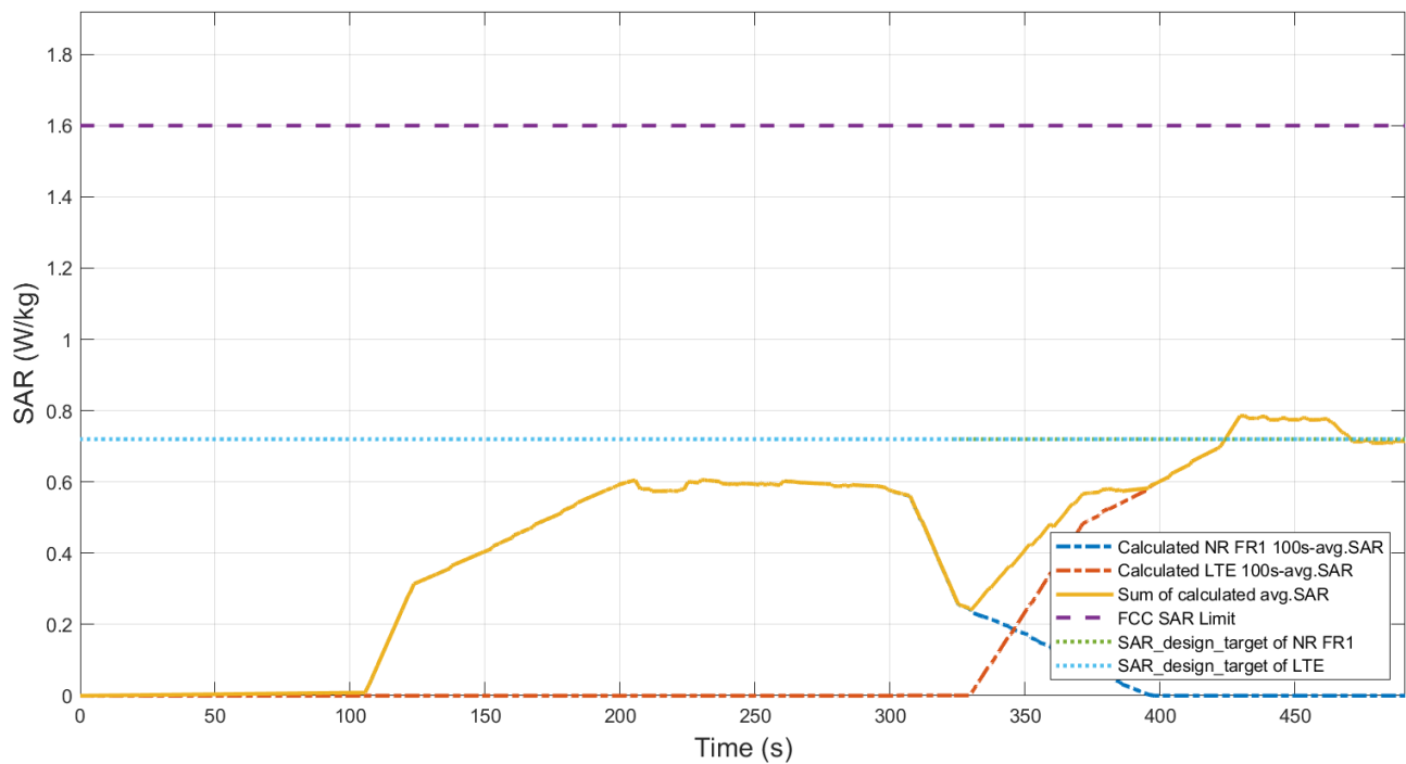
Figure 6.9-2 Total time-averaged SAR
