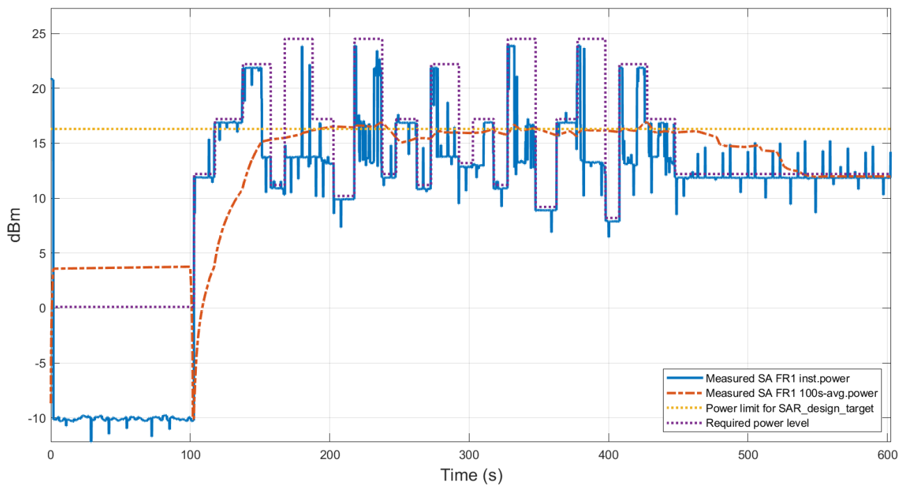
Figure 6.3-7 Conducted Tx power
