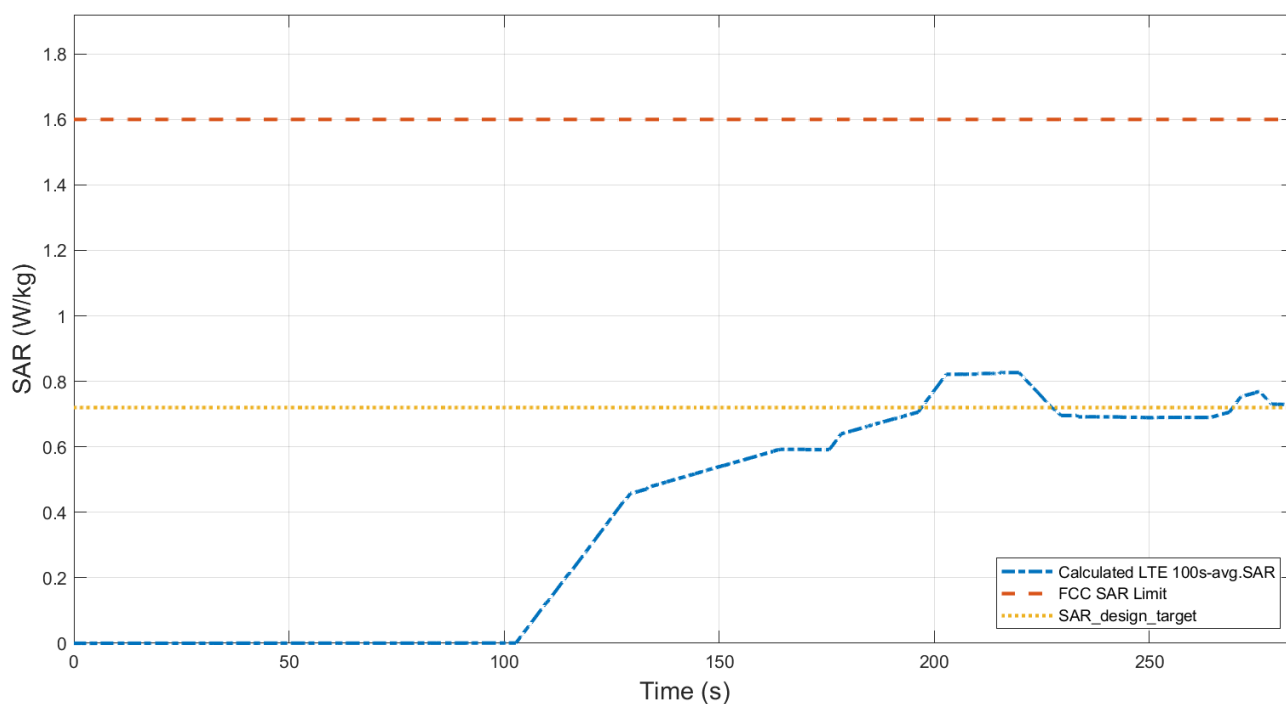
Figure 6.7-2 Total time-averaged SAR
