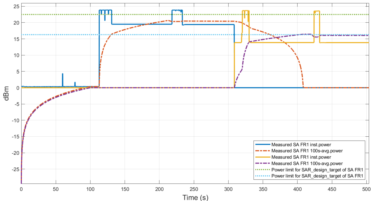
Figure 6.4-1 Conducted Tx power for SAR states change
