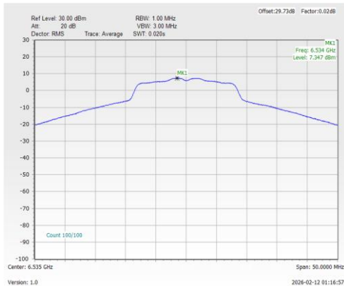
Power Density Plot Trace 2 (Ant 3)
