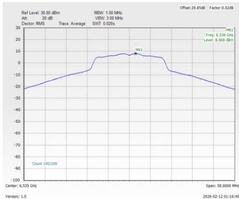
Power Density Plot Trace 1 (Ant 4)
