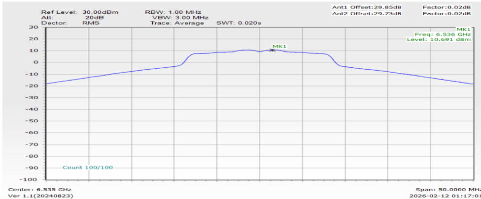
Maximum Power Density Plot (dBm/MHz)
