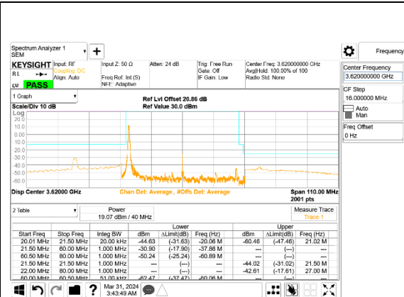
5G NR n48 40MHz BPSK Middle Channel RB1-0, ID:27979
