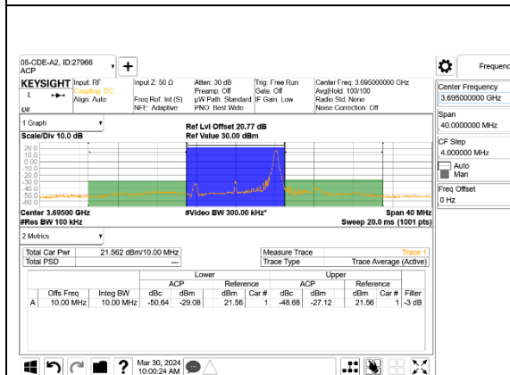
5G NR n48 10MHz BPSK High Channel RB1-23, ID:27966
