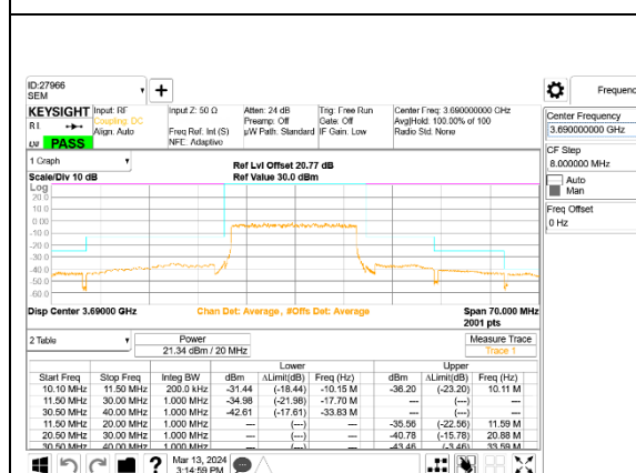
5G NR n48 20MHz BPSK High Channel RB50-0, ID:27966
