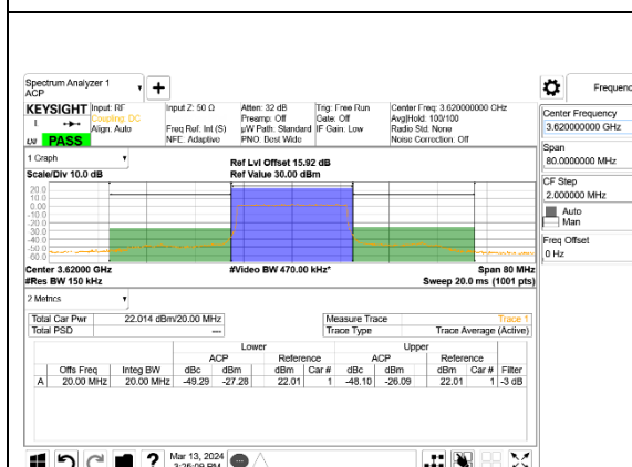
LTE B48 20MHz QPSK Middle Channel RB100-0, ID:39005
