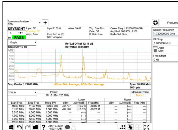
LTE B66B 10MHz + 10MHz QPSK Low Ch RB1-0 + RB1-0
