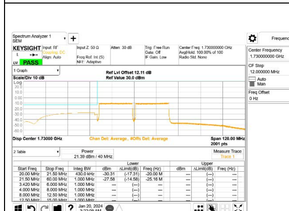
LTE B66C 20MHz + 20MHz QPSK Low Ch RB100-0 + RB100-0
