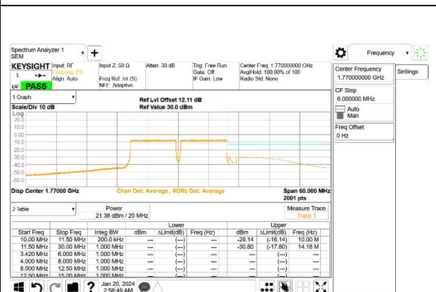
LTE B66B 10MHz + 10MHz QPSK High Ch RB50-0 + RB50-0
