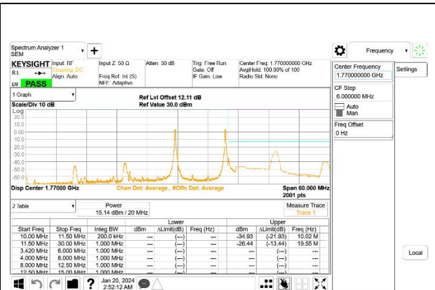
LTE B66B 10MHz + 10MHz QPSK High Ch RB1-49 + RB1-49
