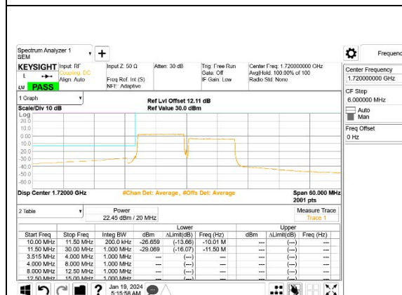
LTE B66B 10MHz + 10MHz QPSK Low Ch RB50-0 + RB50-0
