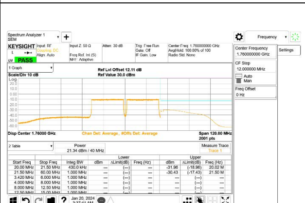
LTE B66C 20MHz + 20MHz QPSK High Ch RB100-0 + RB100-0
