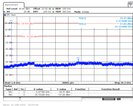
CSE Plot on High Ch between 1GHz ~ 26.5GHz
