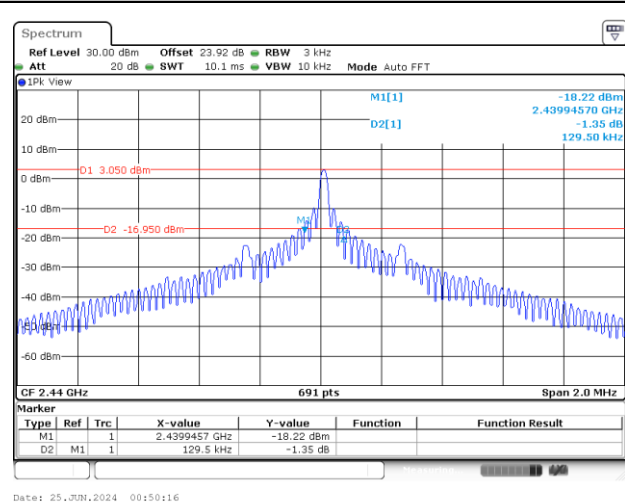
20 dB Bandwidth Plot in Channel 38
