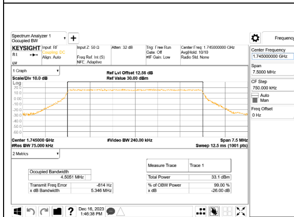
LTE B66 5MHz QPSK Middle Channel RB25-0,ID:39005
