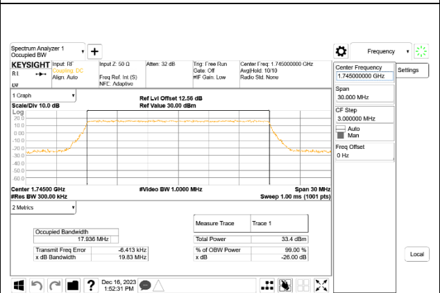
LTE B66 20MHz QPSK Middle Channel RB100-0,ID:39005
