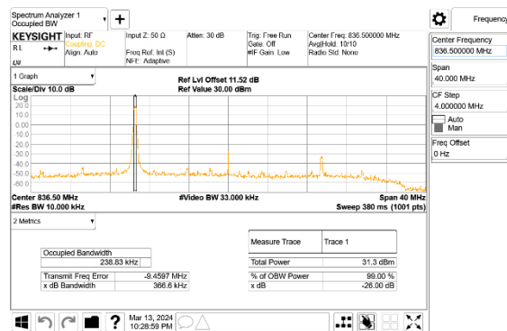
5G NR n26 20MHz Middle High Channel RB1-0,ID:19210
