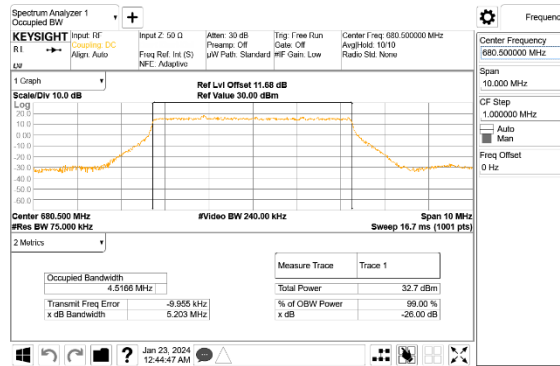
5G NR n71 5MHz BPSK Middle Channel RB25-0, ID:27979
