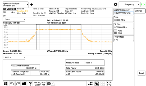
5G NR n48 15MHz BPSK Middle Channel RB36-0, ID:28498
