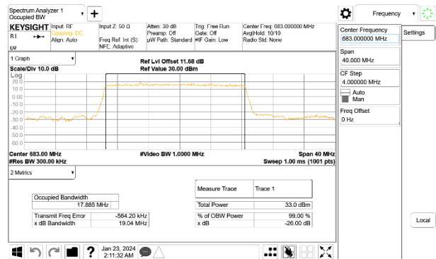
5G NR n71 20MHz BPSK Middle Channel RB100-0, ID:27979
