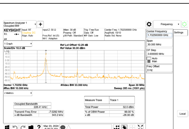
5G NR n70 10MHz BPSK Middle Channel RB1-0,ID:27979
