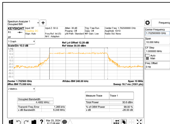
5G NR n70 5MHz BPSK Middle Channel RB25-0,ID:27979
