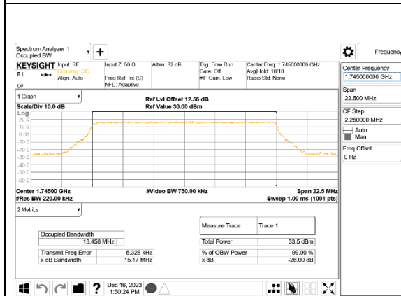
LTE B66 15MHz QPSK Middle Channel RB75-0,ID:39005
