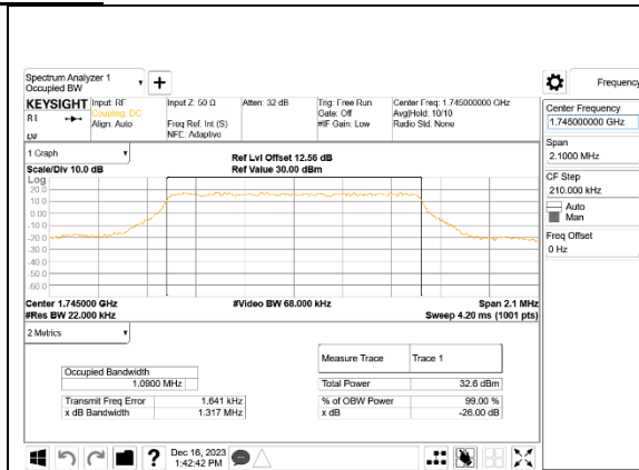
LTE B66 1.4MHz QPSK Middle Channel RB6-0,ID:39005
