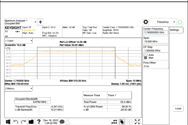
LTE B66 10MHz QPSK Middle Channel RB50-0,ID:39005
