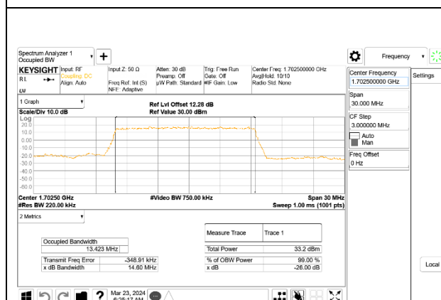
5G NR n70 15MHz BPSK Middle Channel RB75-0,ID:27979
