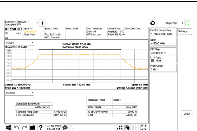
LTE B66 3MHz QPSK Middle Channel RB15-0,ID:39005
