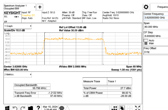
5G NR n48 40MHz BPSK Middle Channel RB100-0, ID:28498
