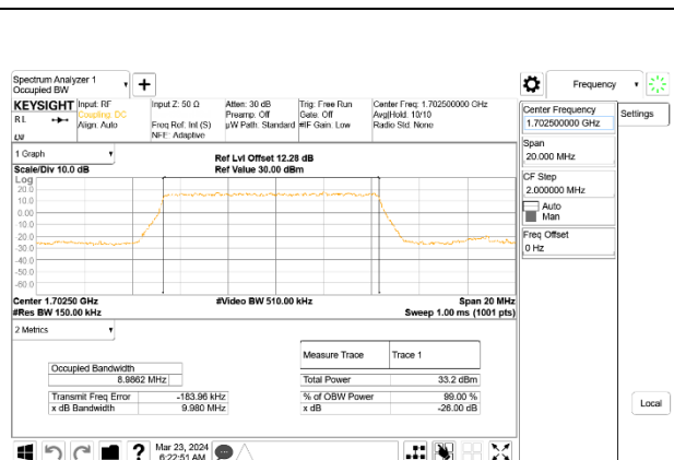
5G NR n70 10MHz BPSK Middle Channel RB50-0,ID:27979
