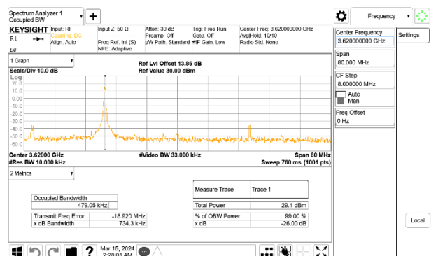
5G NR n48 40MHz BPSK Middle Channel RB1-0, ID:28498
