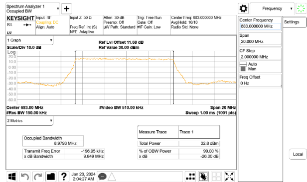
5G NR n71 10MHz BPSK Middle Channel RB50-0, ID:27979
