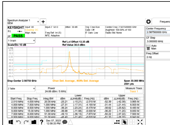
LTE B7 5MHz QPSK High Channel RB1-0, ID:39005
