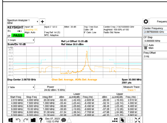
LTE B7 5MHz QPSK High Channel RB1-24, ID:39005
