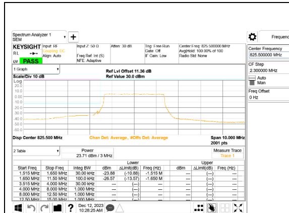
LTE B5 3MHz QPSK Low Channel RB15-0, ID:32061
