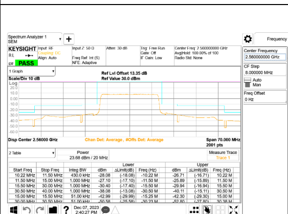
LTE B7 20MHz QPSK High Channel RB100-0, ID:39005
