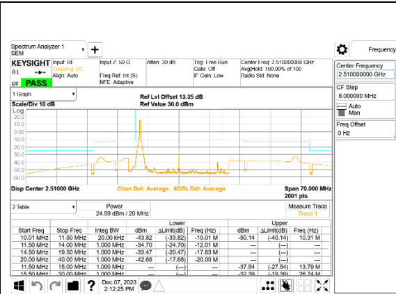
LTE B7 20MHz QPSK Low Channel RB1-0, ID:39005
