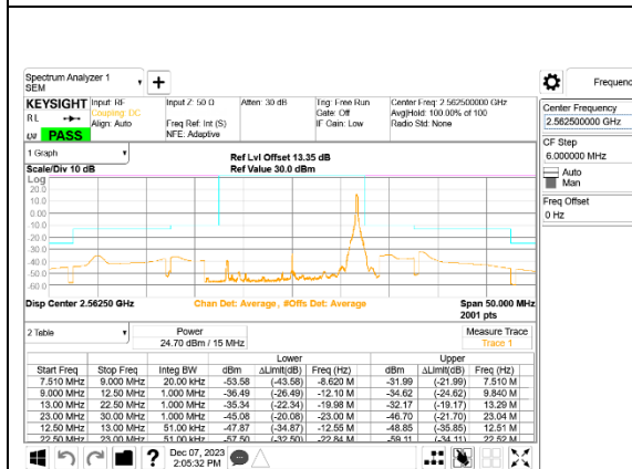
LTE B7 15MHz QPSK High Channel RB1-74, ID:39005
