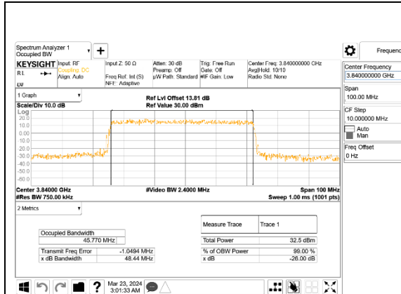
5G NR n77 50MHz BPSK Middle Channel RB128-0, ID:28498
