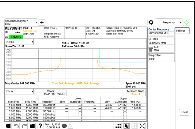
LTE B5 3MHz QPSK High Channel RB15-0, ID:32061
