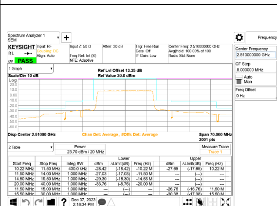
LTE B7 20MHz QPSK Low Channel RB100-0, ID:39005
