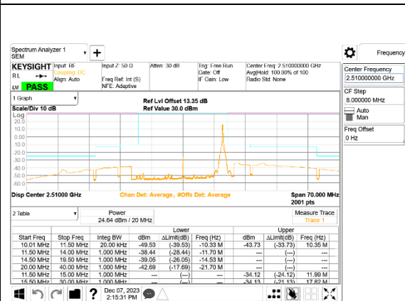
LTE B7 20MHz QPSK Low Channel RB1-99, ID:39005
