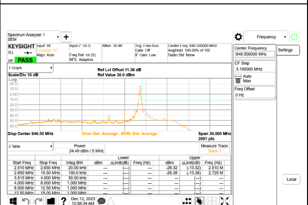
LTE B5 5MHz QPSK High Channel RB1-24, ID:32061
