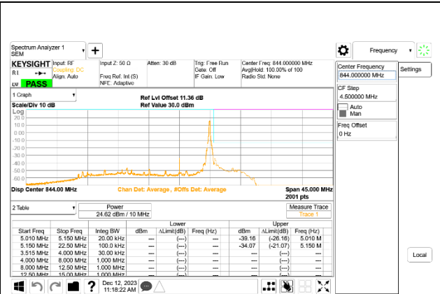
LTE B5 10MHz QPSK High Channel RB1-49, ID:32061
