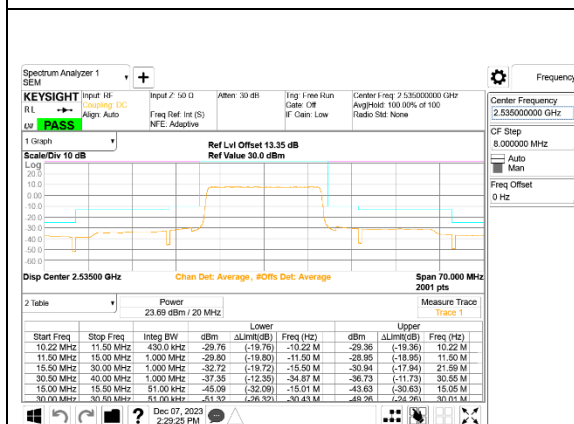
LTE B7 20MHz QPSK Middle Channel RB100-0, ID:39005
