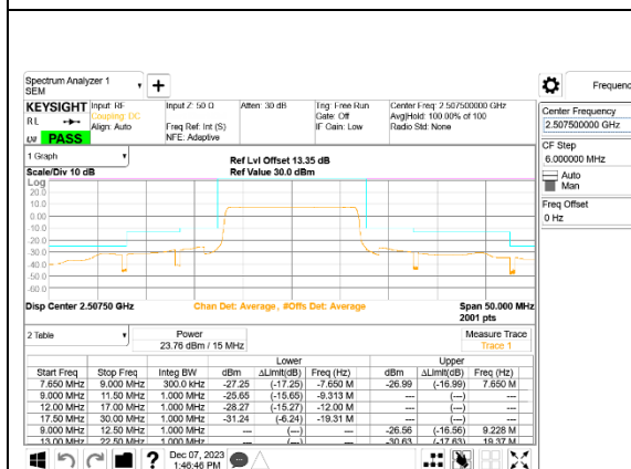
LTE B7 15MHz QPSK Low Channel RB75-0, ID:39005
