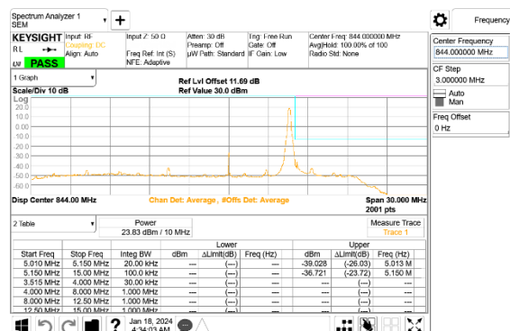
5G NR n5 10MHz BPSK High Channel RB1-51,ID:24898
