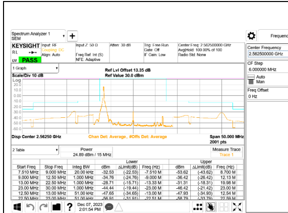
LTE B7 15MHz QPSK High Channel RB1-0, ID:39005
