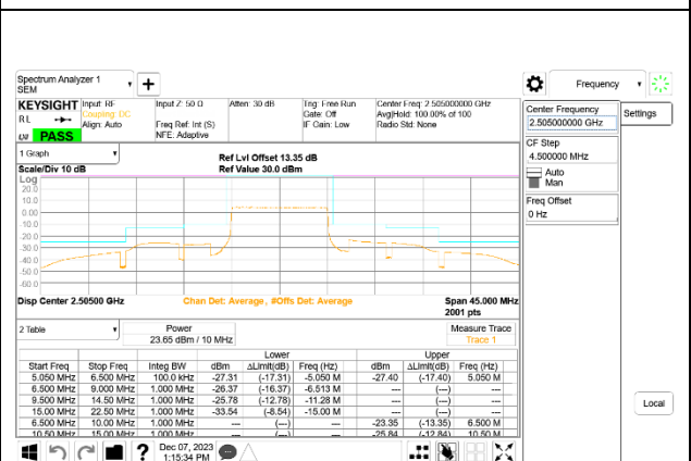
LTE B7 10MHz QPSK Low Channel RB50-0, ID:25780
