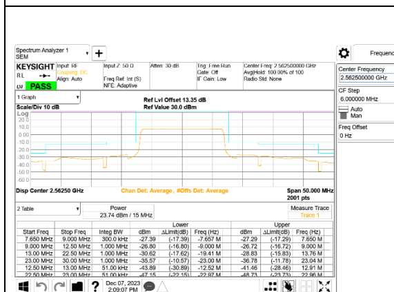
LTE B7 15MHz QPSK High Channel RB75-0, ID:39005
