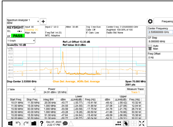
LTE B7 20MHz QPSK Middle Channel RB1-0, ID:39005
