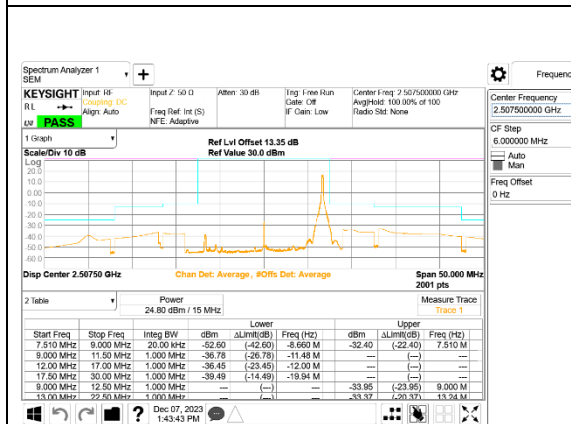
LTE B7 15MHz QPSK Low Channel RB1-74, ID:39005
