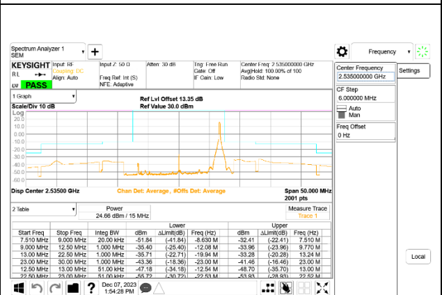
LTE B7 15MHz QPSK Middle Channel RB1-74, ID:39005
