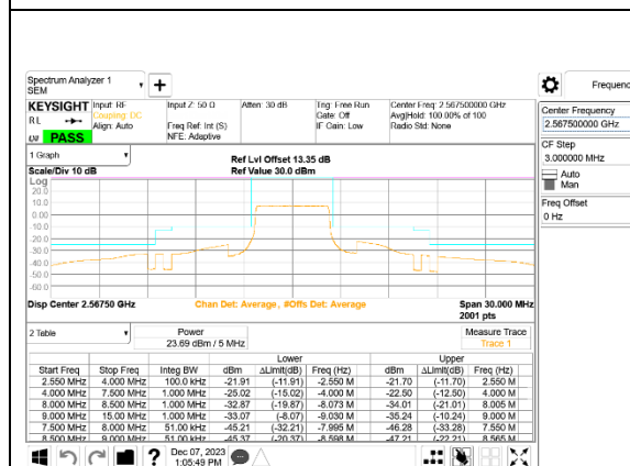
LTE B7 5MHz QPSK High Channel RB25-0, ID:25780
