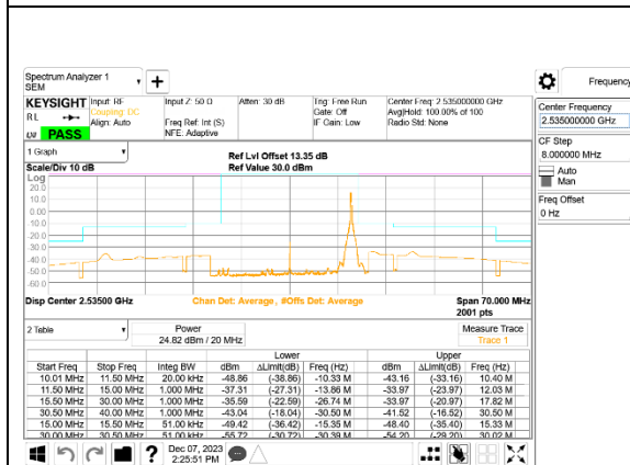
LTE B7 20MHz QPSK Middle Channel RB1-99, ID:39005
