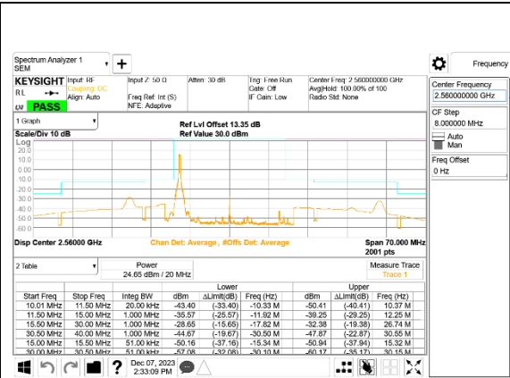
LTE B7 20MHz QPSK High Channel RB1-0, ID:39005
