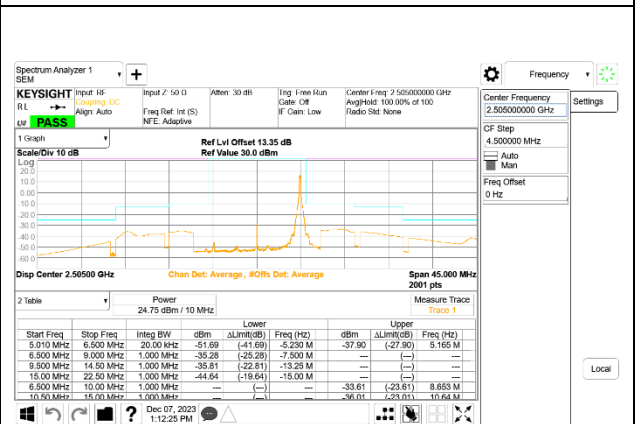
LTE B7 10MHz QPSK Low Channel RB1-49, ID:39005
