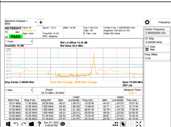
LTE B7 20MHz QPSK High Channel RB1-99, ID:39005
