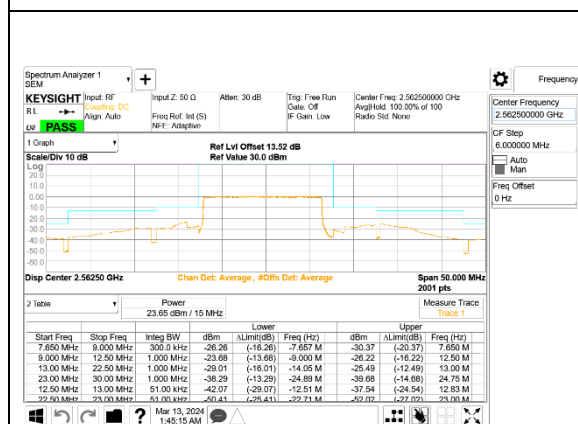
5G NR n7 15MHz BPSK High Channel RB75-0, ID:28498
