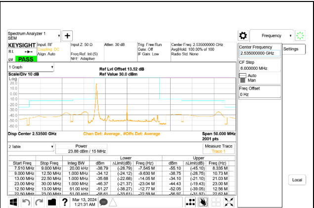
5G NR n7 15MHz BPSK Middle Channel RB1-0, ID:28498
