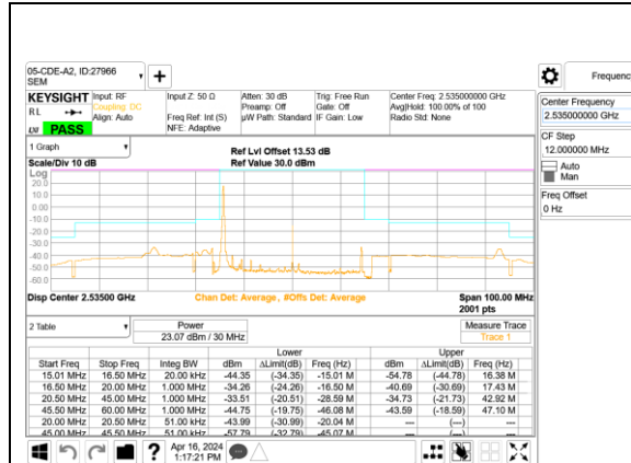
5G NR n7 30MHz BPSK Middle Channel RB1-0
