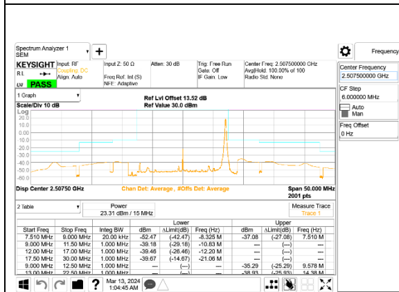
5G NR n7 15MHz BPSK Low Channel RB1-78, ID:28498
