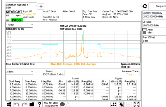
5G NR n7 5MHz BPSK Low Channel RB1-24, ID:28498
