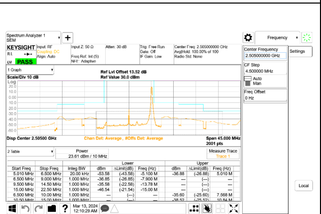
5G NR n7 10MHz BPSK Low Channel RB1-51, ID:28498
