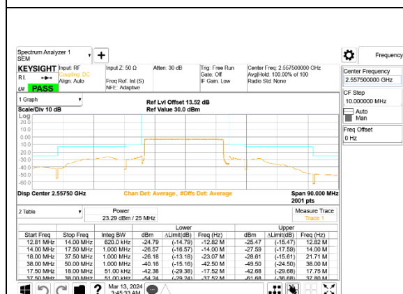
5G NR n7 25MHz BPSK High Channel RB128-0, ID:28498
