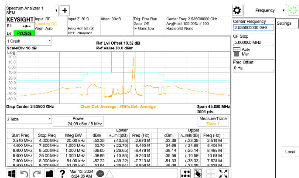
5G NR n7 5MHz BPSK Middle Channel RB1-24, ID:28498
