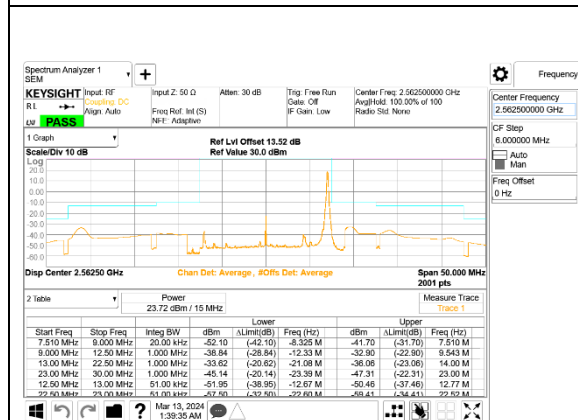
5G NR n7 15MHz BPSK High Channel RB1-78, ID:28498
