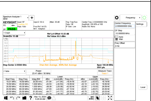
5G NR n7 30MHz BPSK High Channel RB1-159, ID:28498
