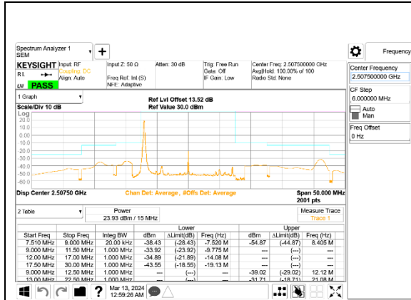
5G NR n7 15MHz BPSK Low Channel RB1-0, ID:28498
