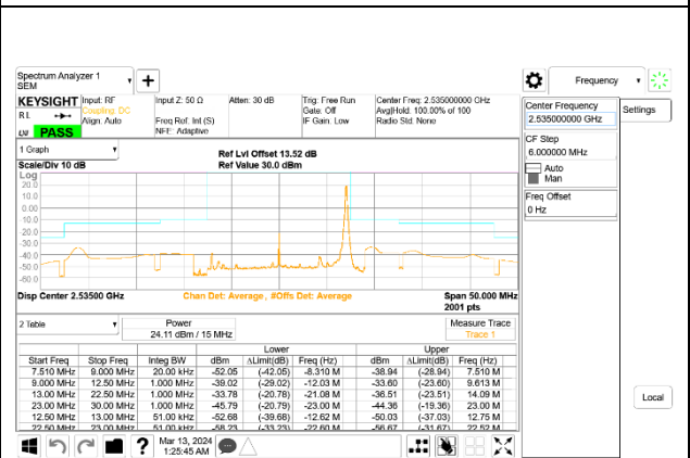
5G NR n7 15MHz BPSK Middle Channel RB1-78, ID:28498
