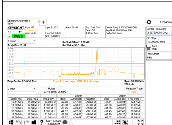
5G NR n7 25MHz BPSK High Channel RB1-132, ID:28498
