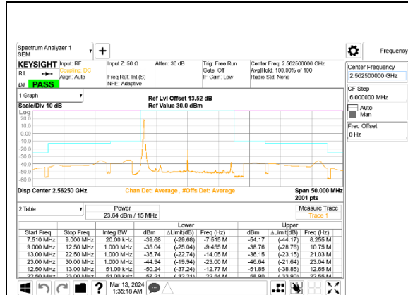
5G NR n7 15MHz BPSK High Channel RB1-0, ID:28498
