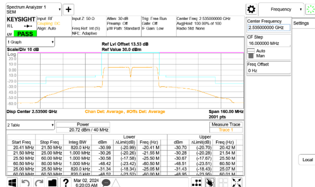
LTE B7 20MHz + 20MHz 16QAM Mid Ch RB100-0 + RB100-0 ID:32061
