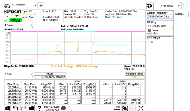
LTE B41 20MHz + 20MHz 16QAM Low Ch RB100-0 + RB100-0 ID:32061
