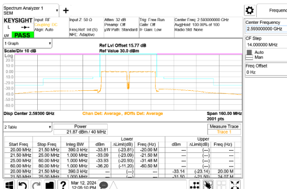
LTE B41 20MHz + 20MHz QPSK Mid Ch RB100-0 + RB100-0 ID:32061
