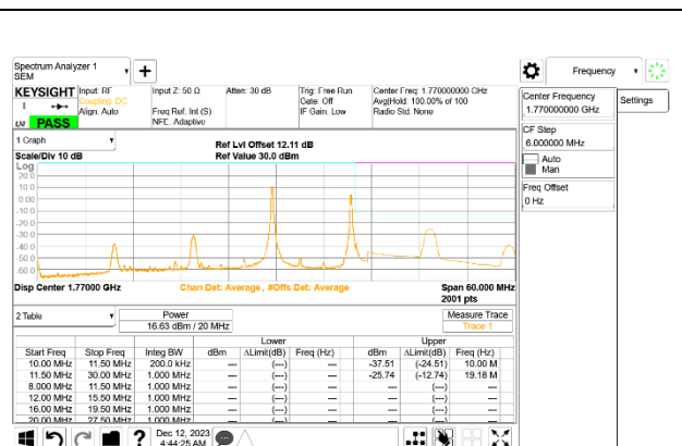
LTE B66B 10MHz + 10MHz 16QAM High Ch RB1-49 + RB1-49 ID:32061
