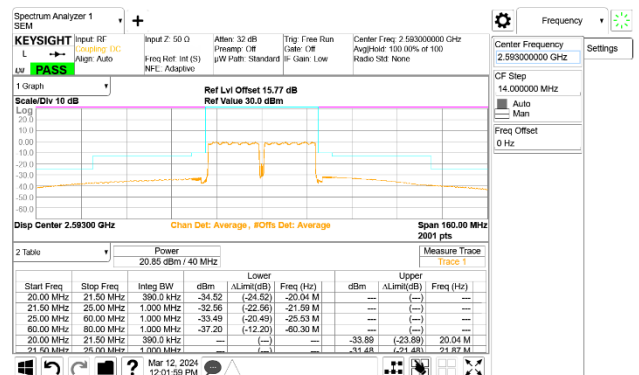
LTE B41 20MHz + 20MHz 16QAM Mid Ch RB100-0 + RB100-0 ID:32061
