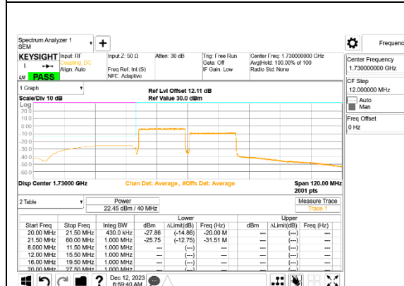
LTE B66C 20MHz + 20MHz QPSK Low Ch RB100-0 + RB100-0 ID:32061
