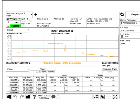
LTE B66B 10MHz + 10MHz QPSK Low Ch RB50-0 + RB50-0 ID:32061
