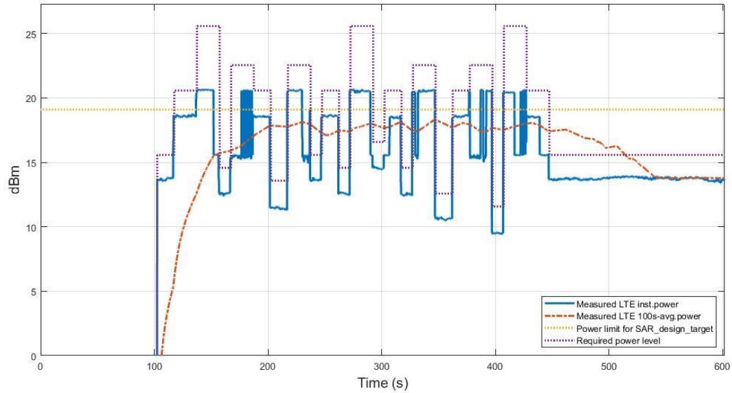
Figure 7.3-9 Conducted Tx power
