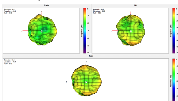
Ant3 Freq. 6475 MHz:
