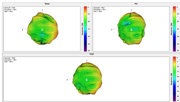
Ant3 Freq. 5887 MHz:
