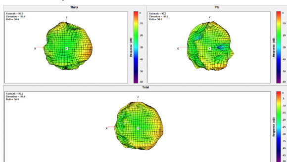
Ant3 Freq. 6175 MHz:
