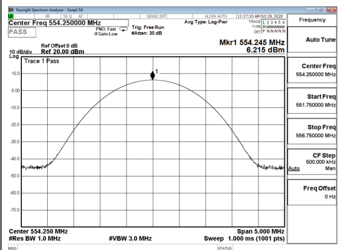
Channel 17 / 554.250 MHz
