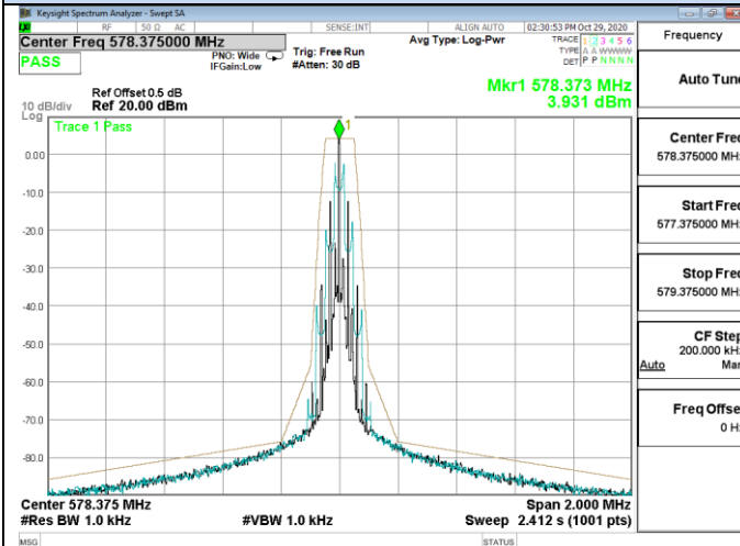
Channel 09 / 578.375 MHz
