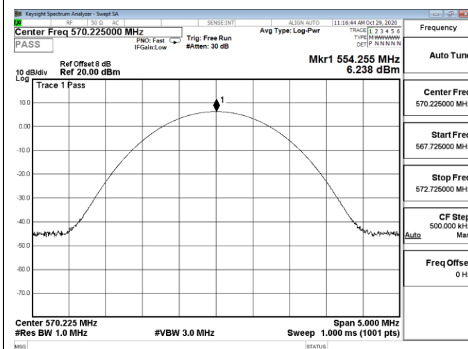
Channel 01 / 570.225 MHz
