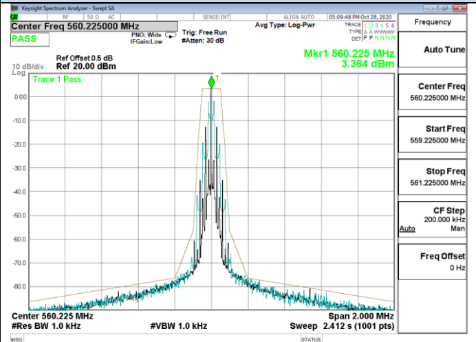
Channel 25 / 560.225 MHz
