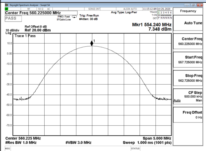
Channel 25 / 560.225MHz
