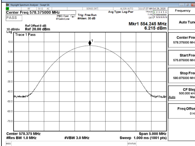
Channel 09 / 578.375MHz
