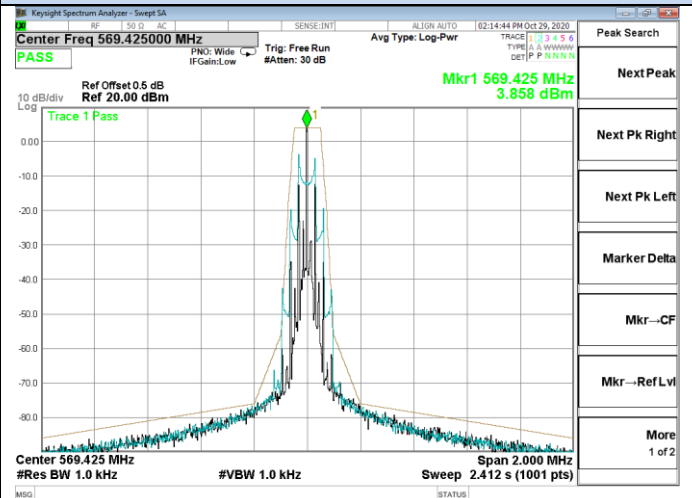
Channel 32 / 569.425 MHz
