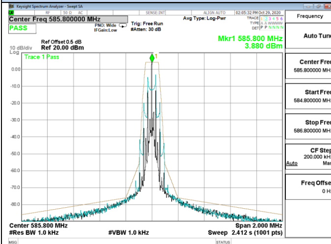
Channel 16 / 585.800 MHz
