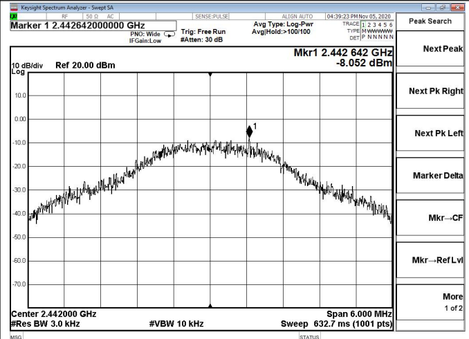
Channel 3 / 2442 MHz
