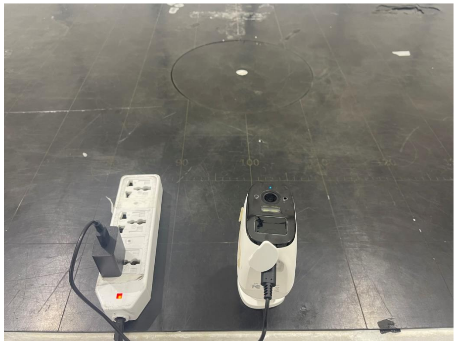
Radiation Emission Test Setup (30MHz to 1GHz) (TM1)
