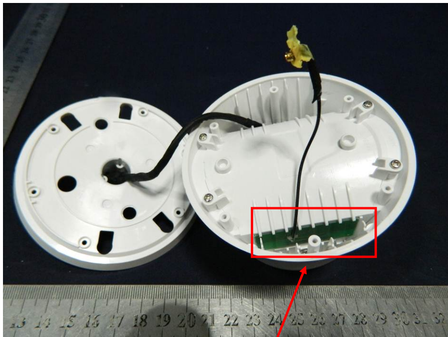
Antenna1
