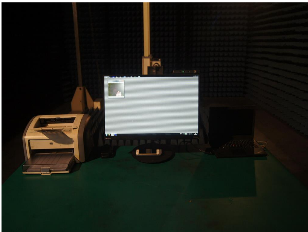
Photograph 2: Set-up for Radiated Emissions (1GHz-6GHz)
