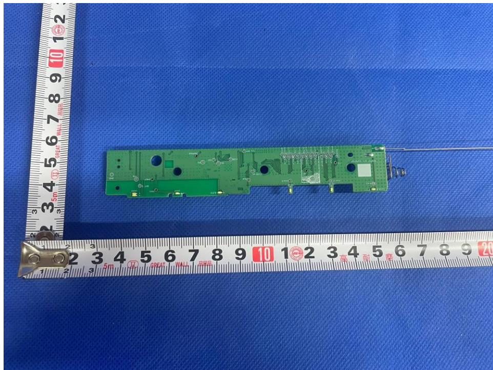
Fig. 4 Bottom view of mainboard
