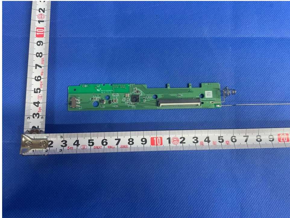
Fig. 3 Top view of mainboard
