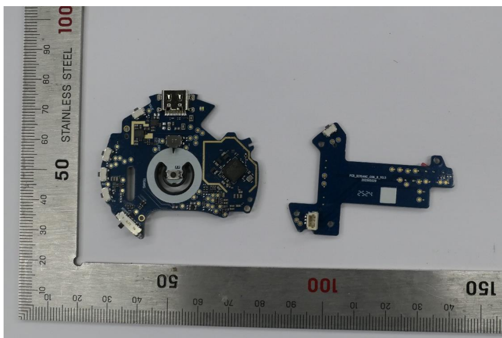
Figure 4: PCB view of headset
