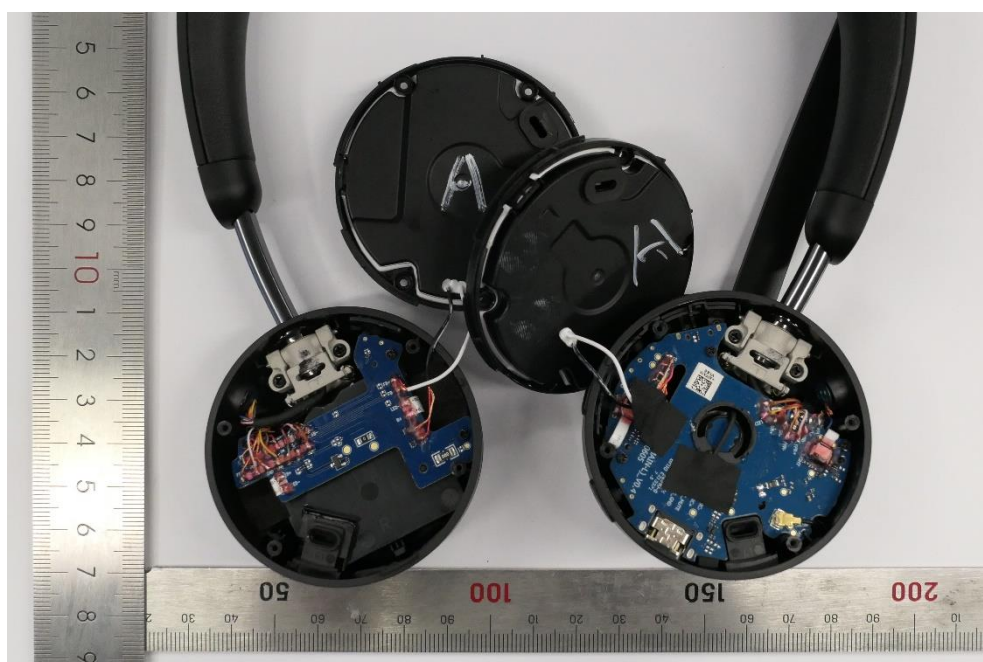
Figure 2: Internal view of headset
