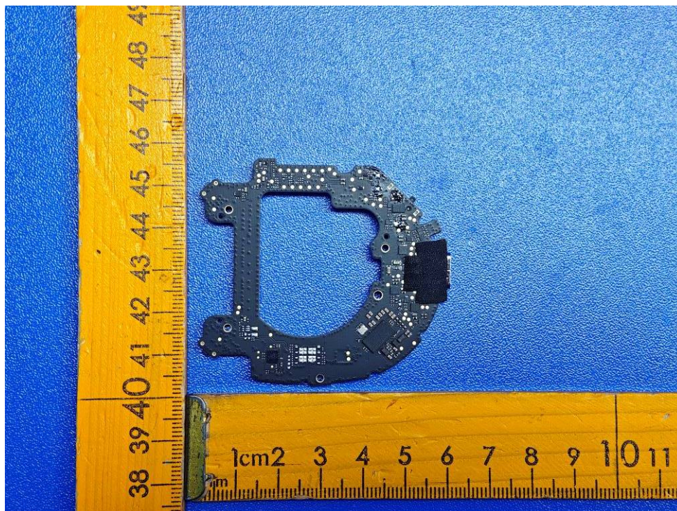
Figure 5: Bottom view of main board 1
