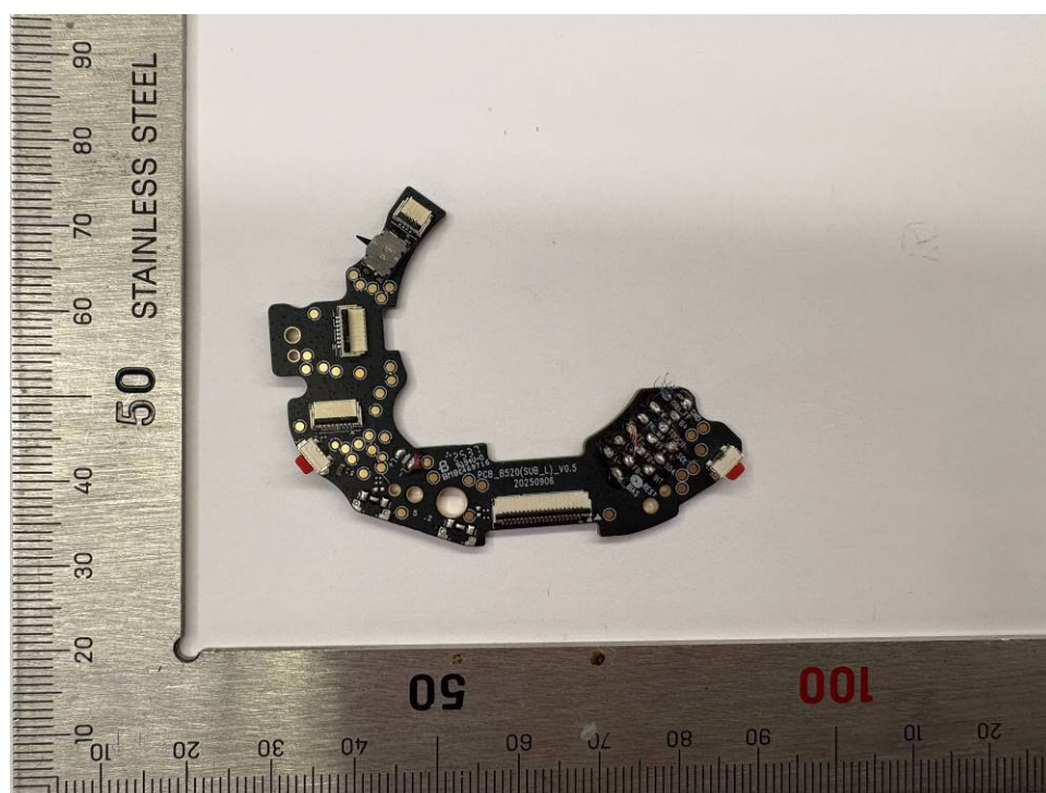
Figure 6: Top view of main board 2
