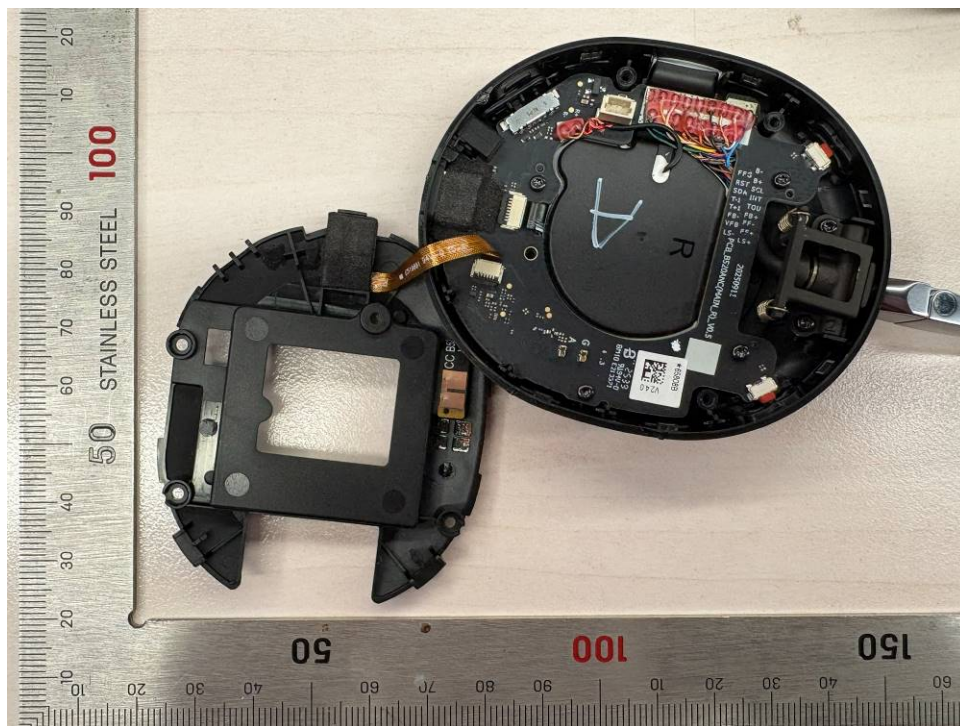
Figure 3: Internal view of EUT
