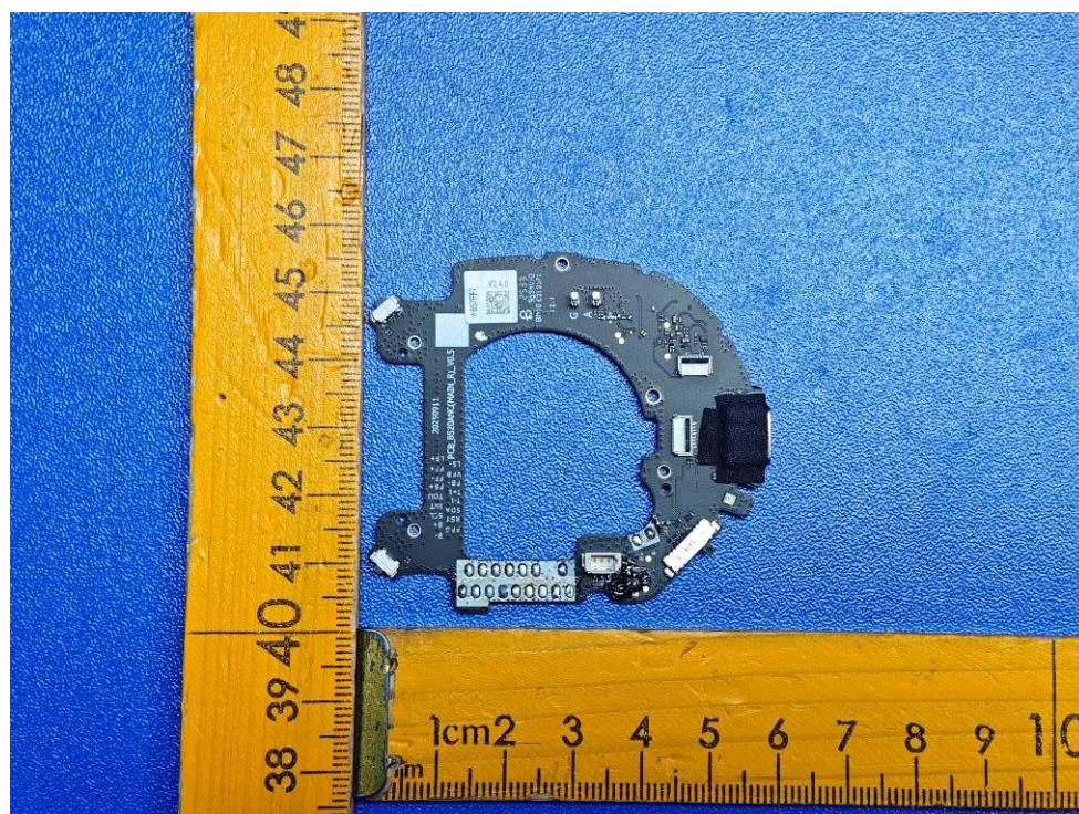
Figure 4: Top view of main board 1
