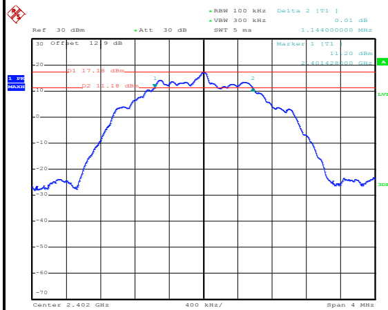
6 dB Bandwidth Plot on Channel 00
