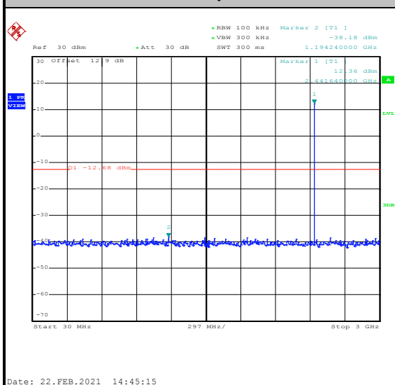
Conducted Spurious Emission Plot on Bluetooth LE 2Mbps GFSK Channel 19
