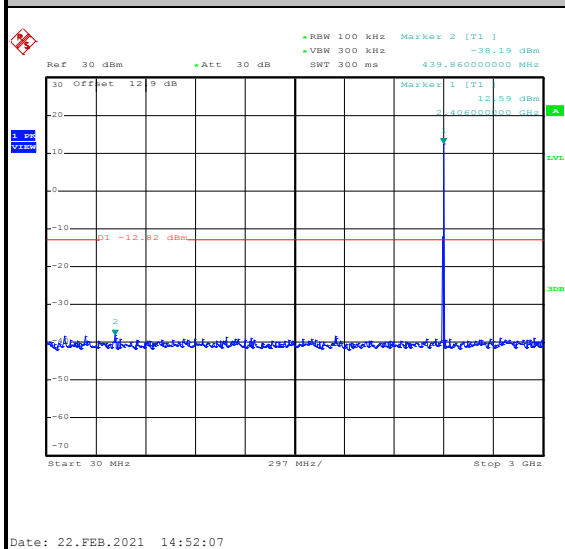
Conducted Spurious Emission Plot on Bluetooth LE 2Mbps GFSK Channel 00
