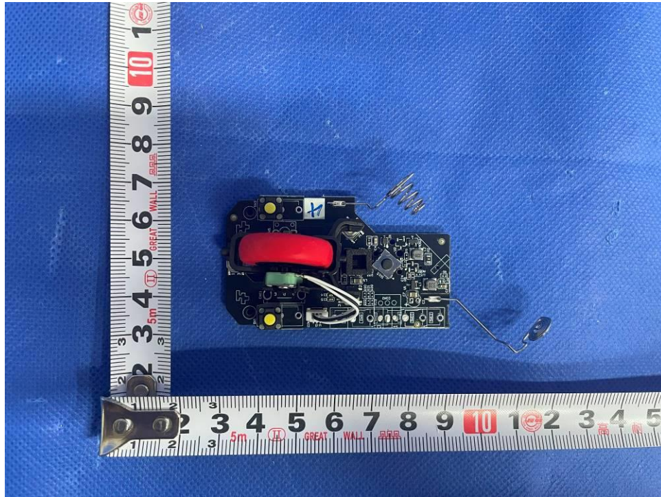
Fig. 7 Top view of mainboard (Product No.: MB565T)
