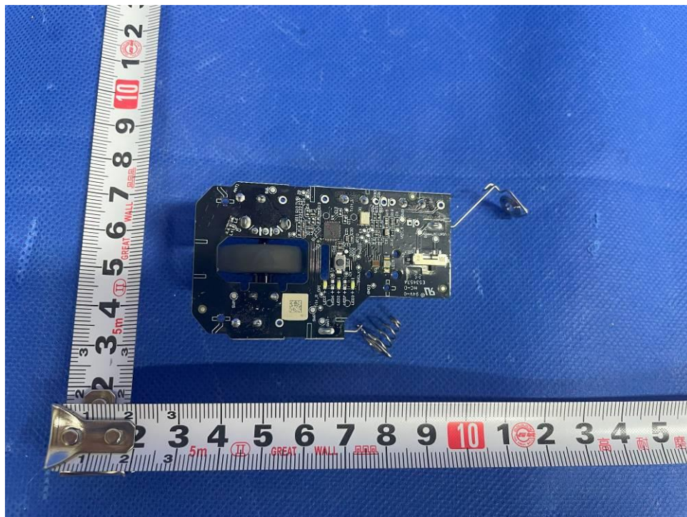
Fig. 4 Bottom view of mainboard (Product No.: MB231T)
