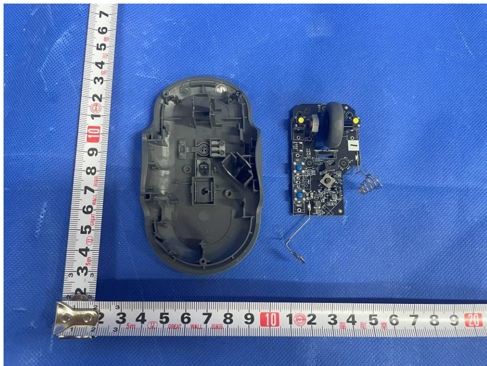
Fig. 2 Internal view (Product No.: MB231T)
