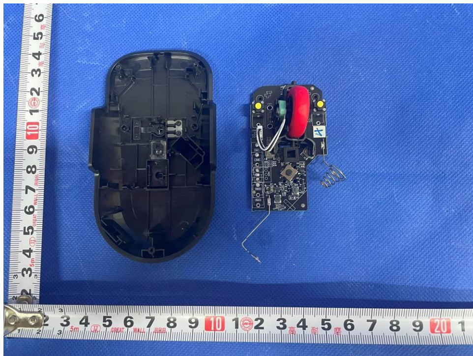
Fig. 6 Internal view (Product No.: MB565T)
