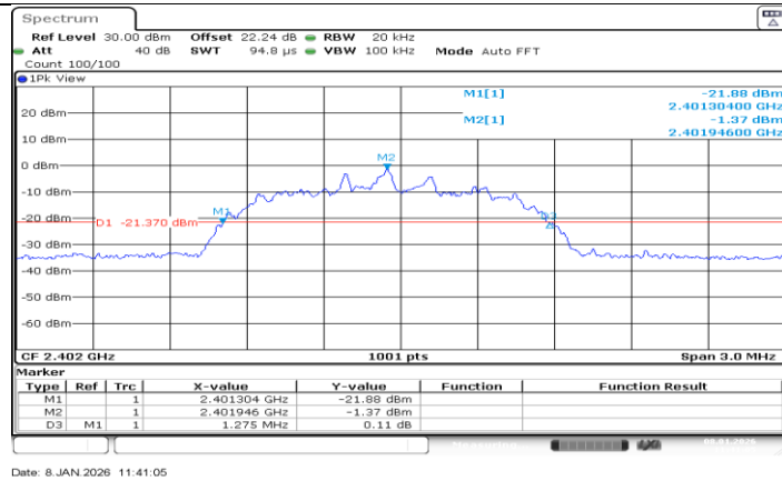
2DH5 Ant1_2402
