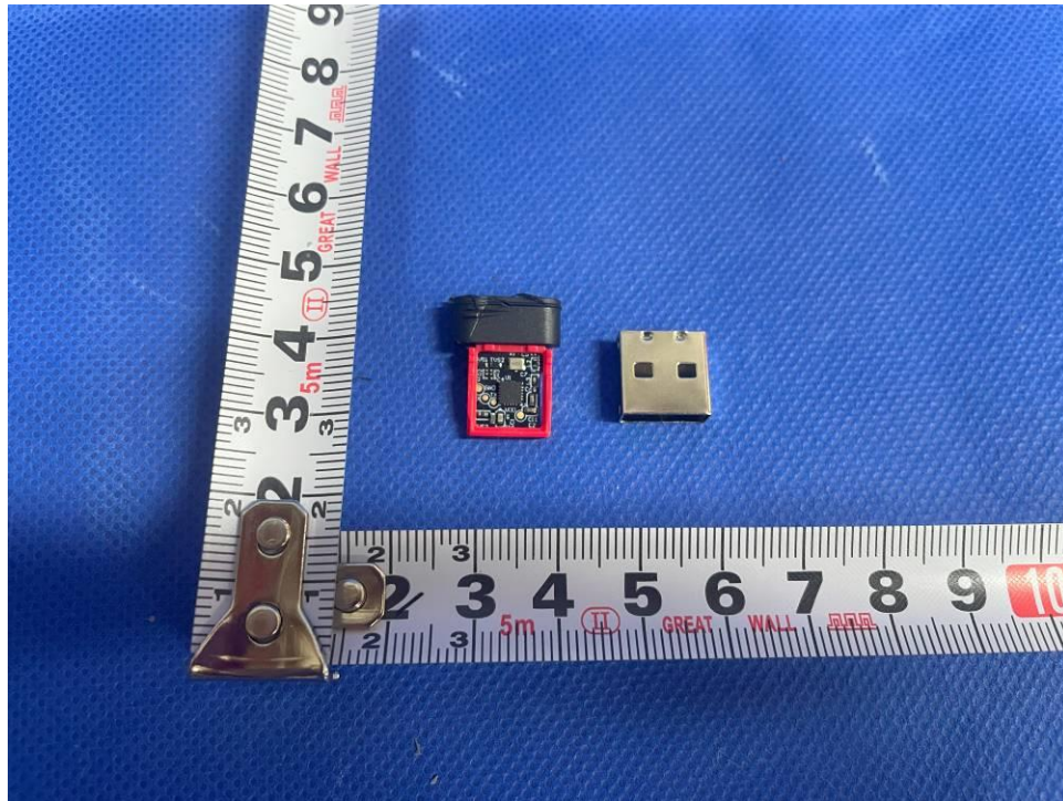
Figure 1: Internal view
