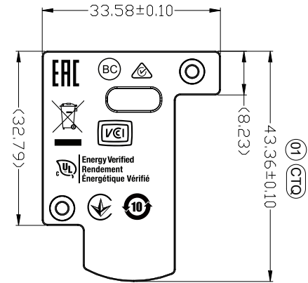
Molding layout
