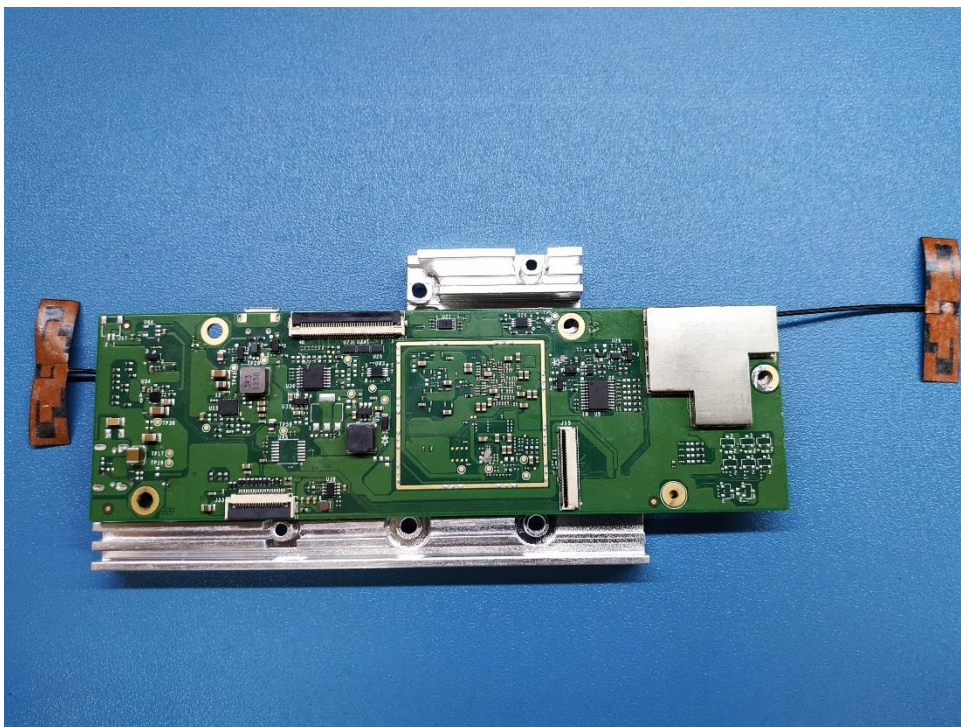
Photo 10: EUT bottom view with Molex antenna
