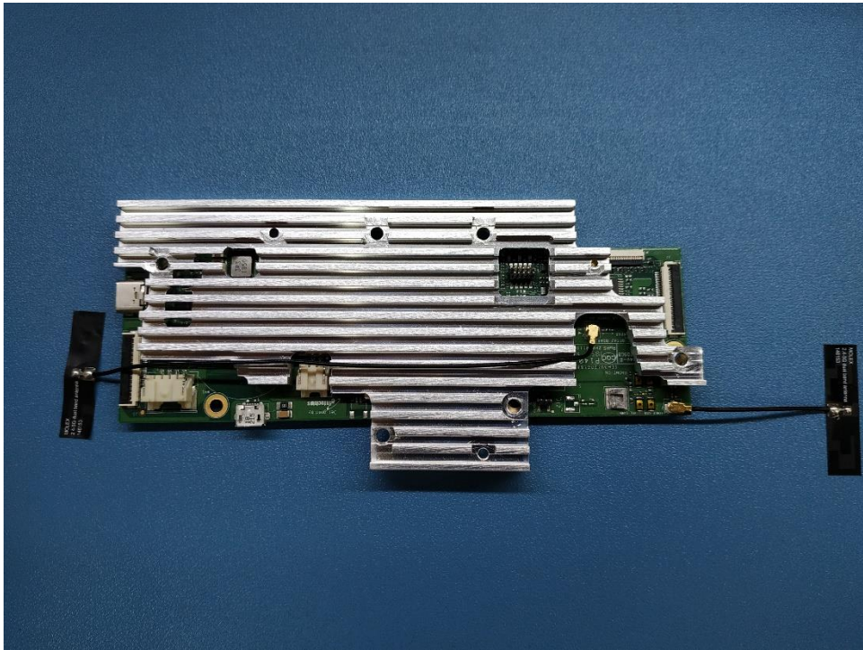
Photo 9: EUT top view with Molex antenna
