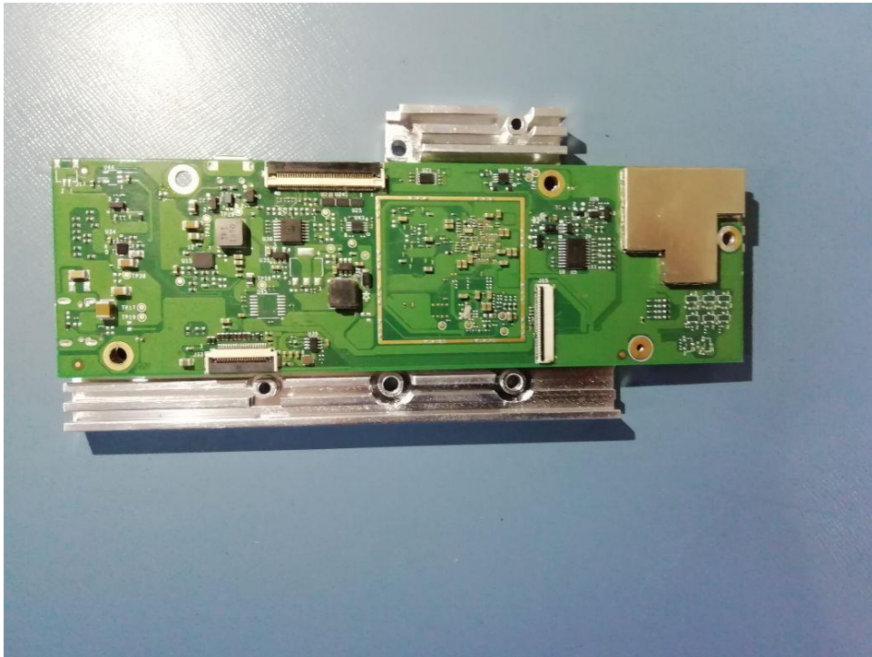
Photo 3: Stand alone module top view ( without antenna)
