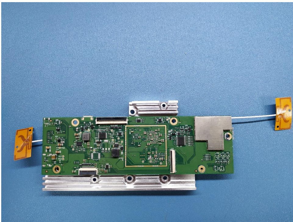
Photo 8: EUT Bottom view with Antennova antenna
