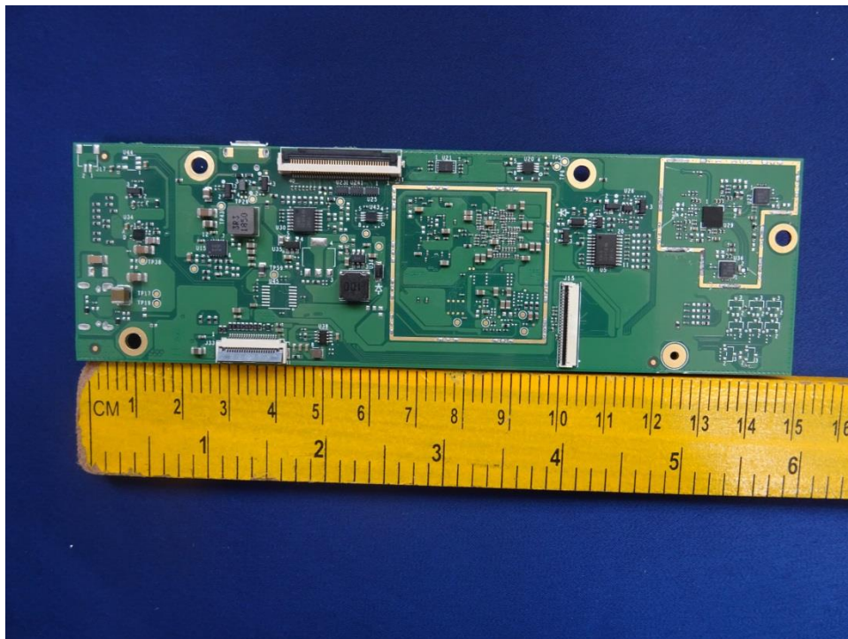
Photo 3: EUT Dimensional view
