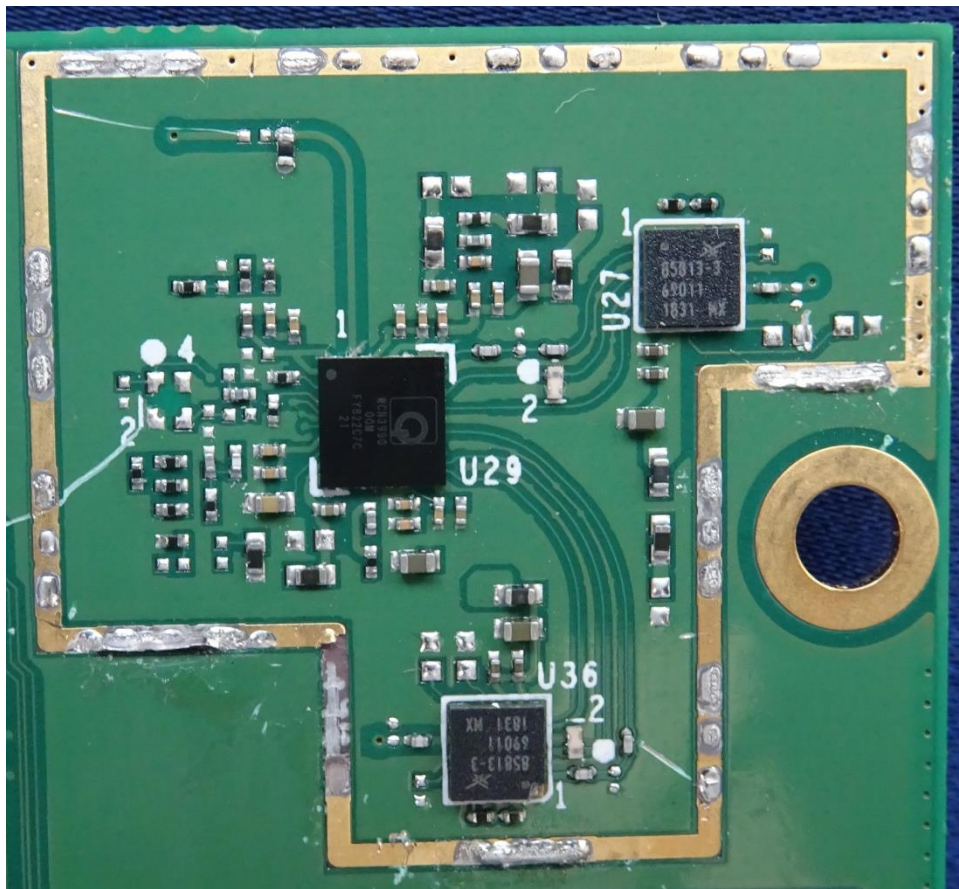
Photo 5: Radio Part
