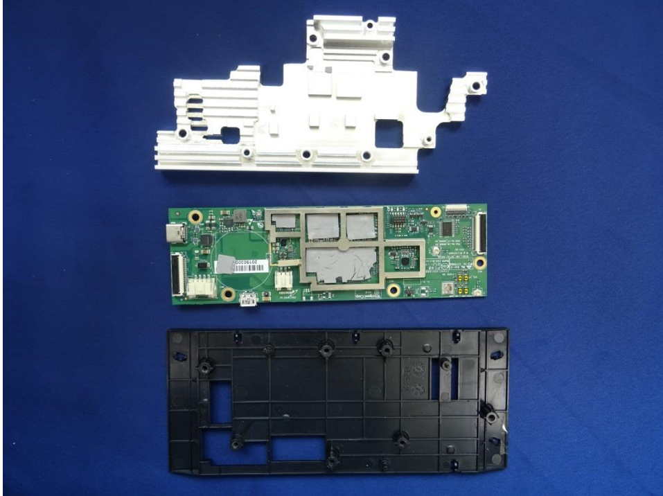
Photo 1: EUT with heatsink and back pannel removed
