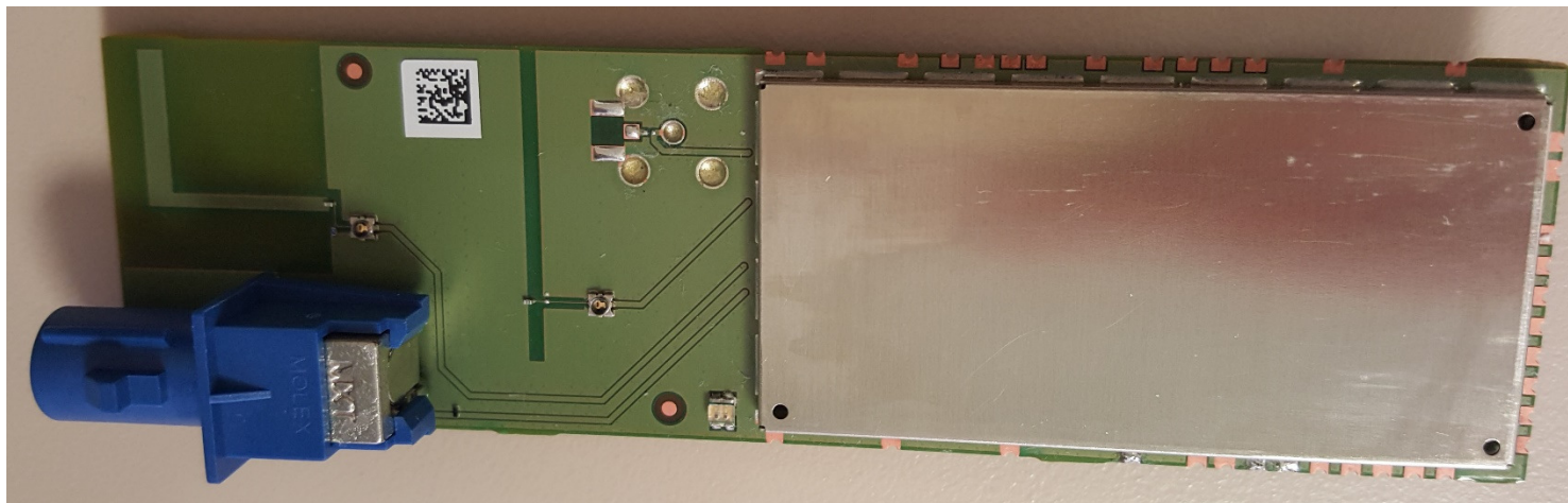
Circuit Board with RF Shield – Side 1
