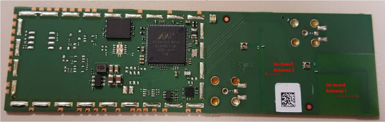
Circuit Board with On-board Antenna Configuration – Side 1 with Shield Removed
