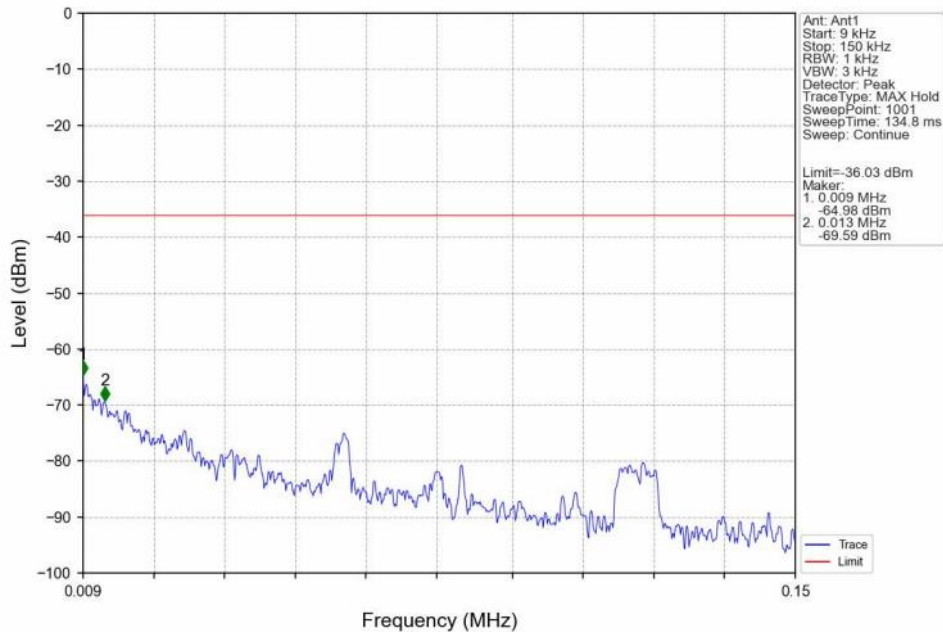
Pi/4DQPSK_2DH5_LCH_2402MHz_Ant1_NTNV
