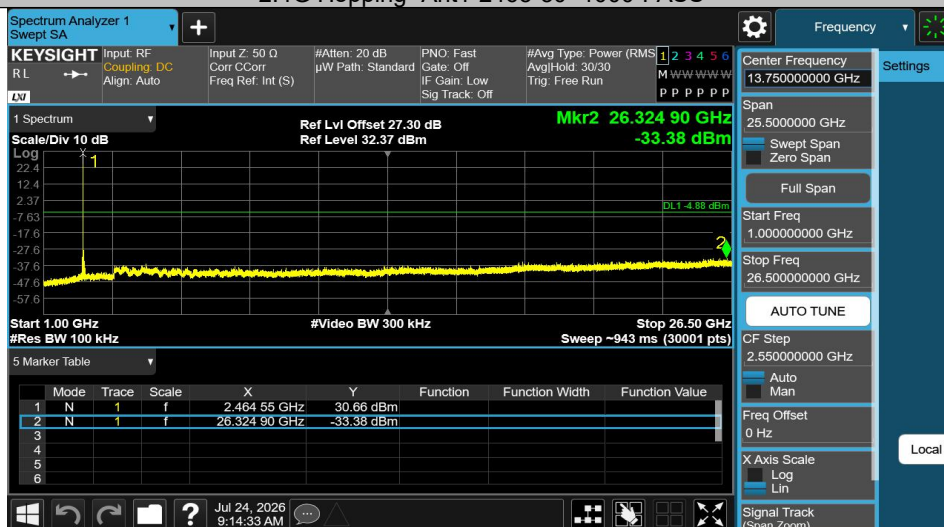
2.4G Hopping -Ant1-2465-1000~26500-PASS
