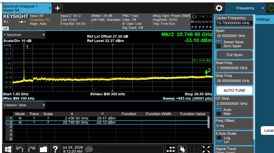
2.4G Hopping -Ant1-2437-1000~26500-PASS
